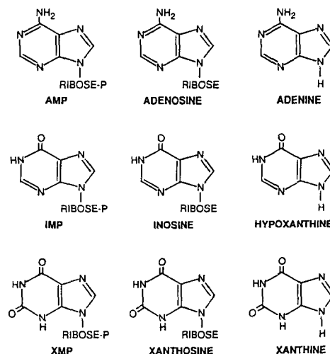
Figure 2. Structure of purine nucleotides, ribosides, and bases.
