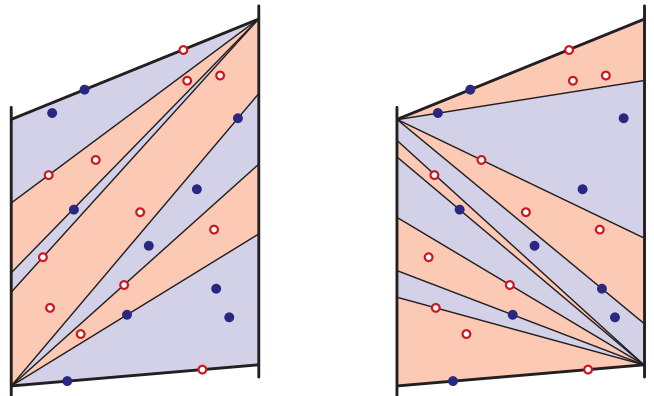
Figure 4. T(t^-, t^+, \text{left}) = 6 and T(t^-, t^+, \text{right}) = 8 .
