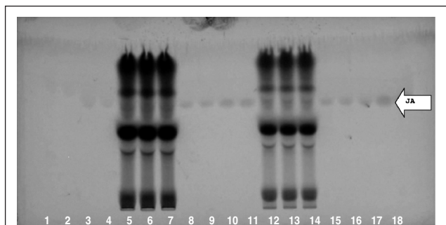
Figure 1. Sample and standard JA were loaded onto silica gel 60 F_{254} TLC foils and run in I–A–W [10:1:1 (v/v)] and the foil was exposed to UV light. Track 1 and 2 = 6 \mu\text{g} of JA; Track 3 and 4 = 10 \mu\text{g} of JA; Track 5, 6, and 7 = 10 \mu\text{L} sample; Track 8 and 9 = 20 \mu\text{g} of JA; Track 10 and 11 = 40 \mu\text{g} of JA; Track 12, 13, and 14 = 5 \mu\text{L} sample; Track 15 and 16 = 60 \mu\text{g} of JA; Track 17 and 18 = 90 \mu\text{g} of JA.
