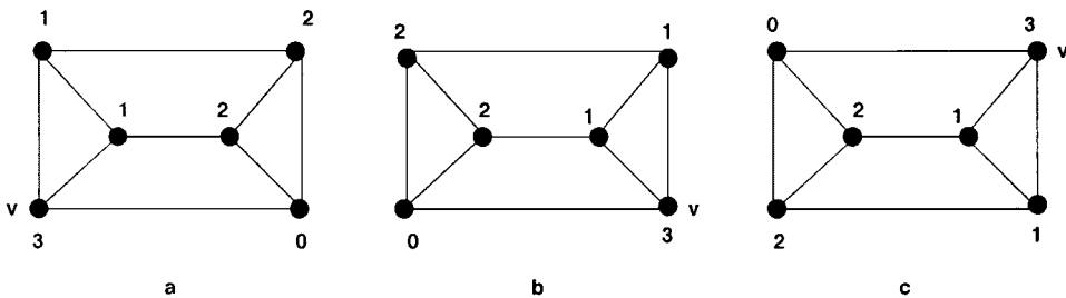
Figure 1. Probing from vertex v .
