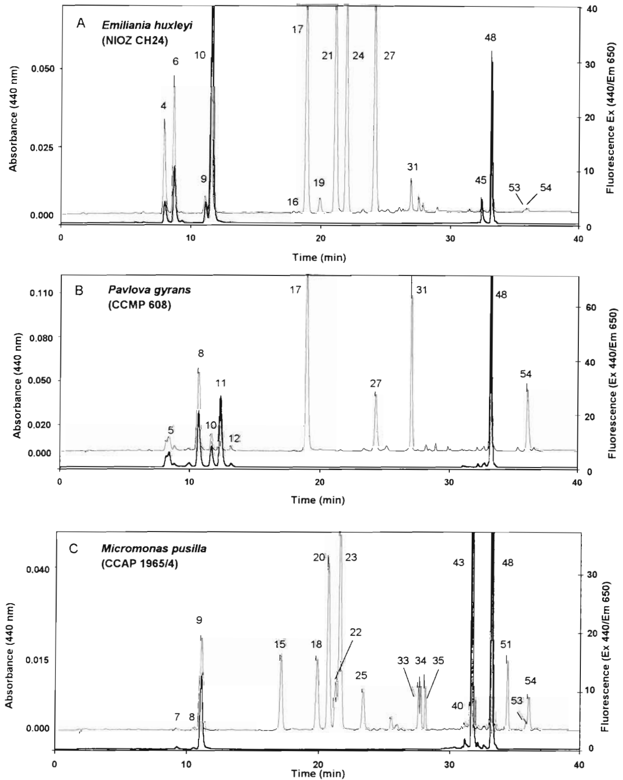
Fig. 2. Pigment composition from the algal cultures (A) Emiliana huxleyi NIOZ CH 24, (B) Pavlova gyrans CCMP 608, (C) Micromonas pusilla CCAP 1965/4, (D) Pelagococcus subviridis CCMP 1429, (E) Skeletonema costatum Sk-1-CIMA, (F) Dunaliella tertiolecta ICMA, (G) Rhodomonas baltica ICMA, (H) Prochlorococcus marinus CCMP 1375, (the insert shows a chromatogram of a mixture of P. marinus and D. tertiolecta ICMA obtained by using a modified gradient profile), (I) Alexandrium minutum ALI 9-IE, and (J) Tetraselmis suecica ICMA. HPLC System 1. Detection by absorbance at 440 nm (thin trace) and fluorescence at Ex 440/Em 650 nm (thick trace). Peak identifications as in Table 2
