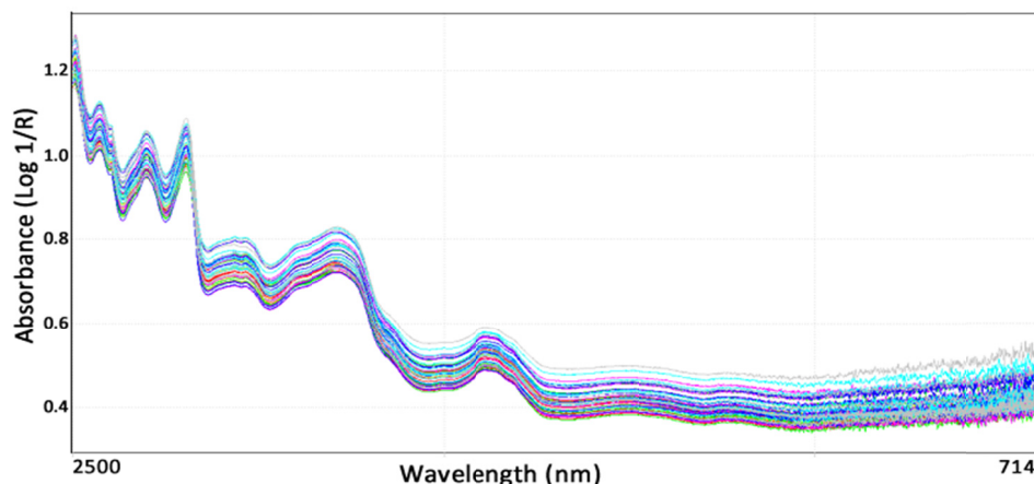
Figure 2. Sixty original spectra in the range near-infrared acquired of the samples
