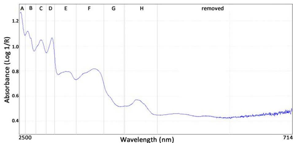
Figure 1. Near-infrared spectrum of a raw soybean seed. Letters delimit sectors of the spectrum. The wavelengths of the sectors appear in Table 1
