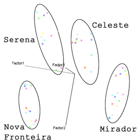
Figure 6. Separation of the four soybean cultivars by the PCA technique
