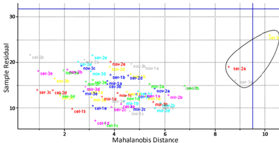
Figure 4. Identification of the anomalous samples by the PCA
