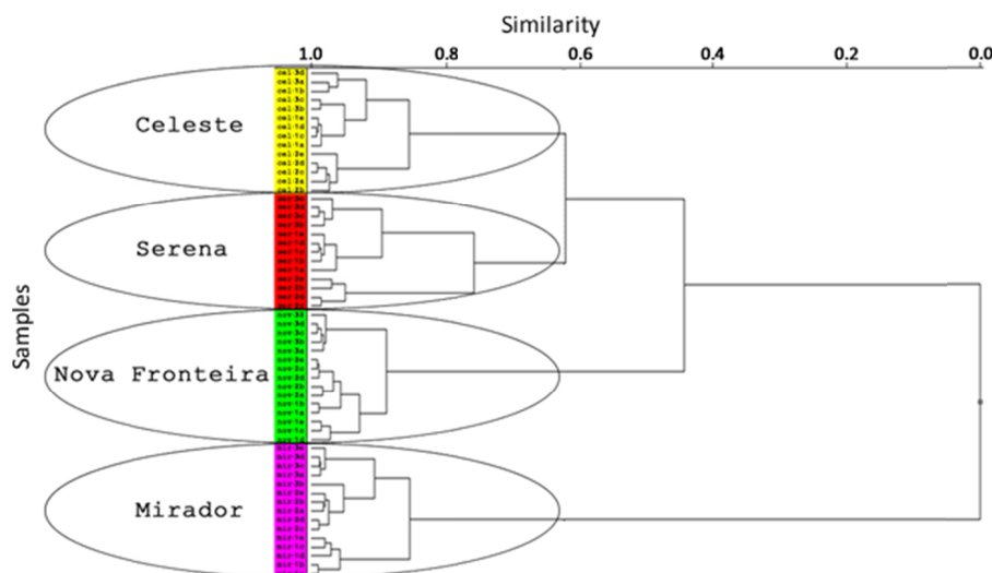
Figure 5. Separation of the four soybean cultivars by the HCA technique
