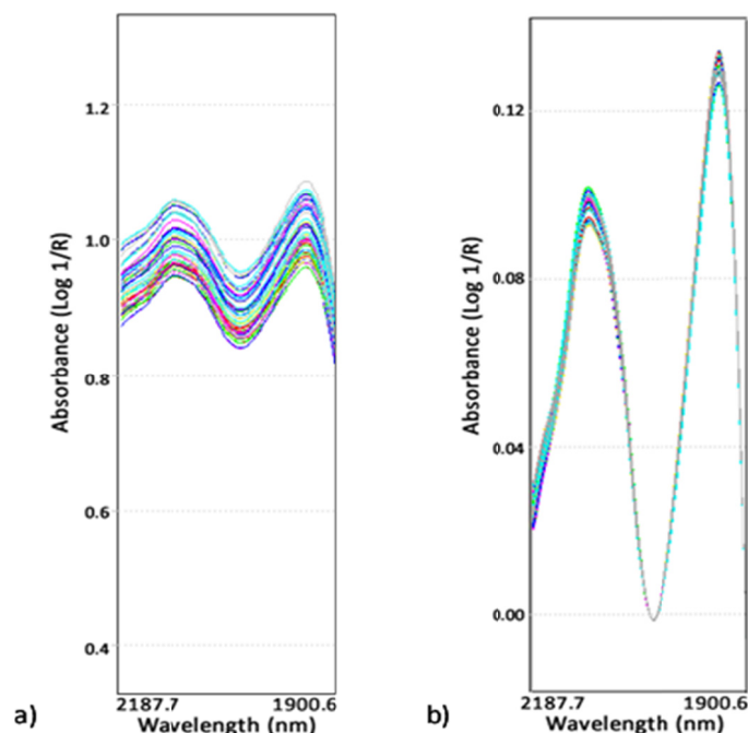
Figure 3. Spectral range with better chemometric results (regions C and D from 1900.6 to 2187.7 nm): a) without treatment and b) with treatment using Multiplicative Signal Correction + Baseline Correct (linear fit)
