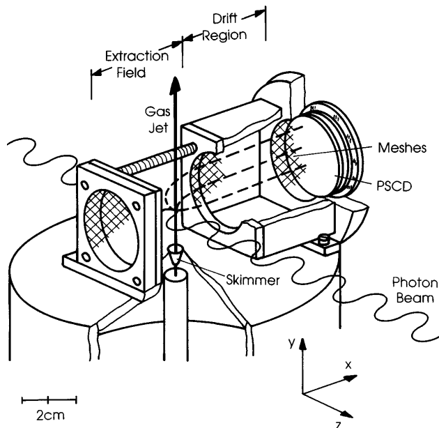
FIG. 1. Recoil-ion momentum spectrometer with supersonic He gas jet. The recoil ions have been measured in coincidence with the beam pulse, the channel-plate detector (PSCD) is two-dimensional position sensitive with wedge and strip readout. The electric field vector of the linear polarized light is parallel to the extraction field.
