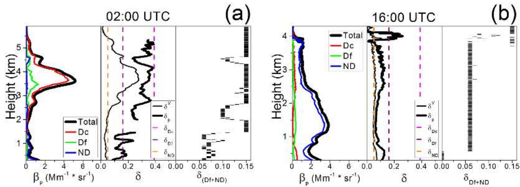
Figure 4. Dust event on 5 July 2016. Vertical profiles of the particle backscatter coefficients (total and for each specific component; left panels), the linear depolarization ratios (volume \delta^V and particle \delta_p ; centre panels) and the estimated depolarization ratio for the fine (Df + ND) mode ( \delta_{Df+ND} ; right panels) at two time intervals, illustrating the different aerosol scenarios observed throughout the day: (a) at 02:00 UTC (high dust incidence) and (b) at 16:00 UTC (low dust incidence). Specific depolarization ratios selected for each pure aerosol component are also shown by vertical dashed lines (see legend) in the centre panels.
