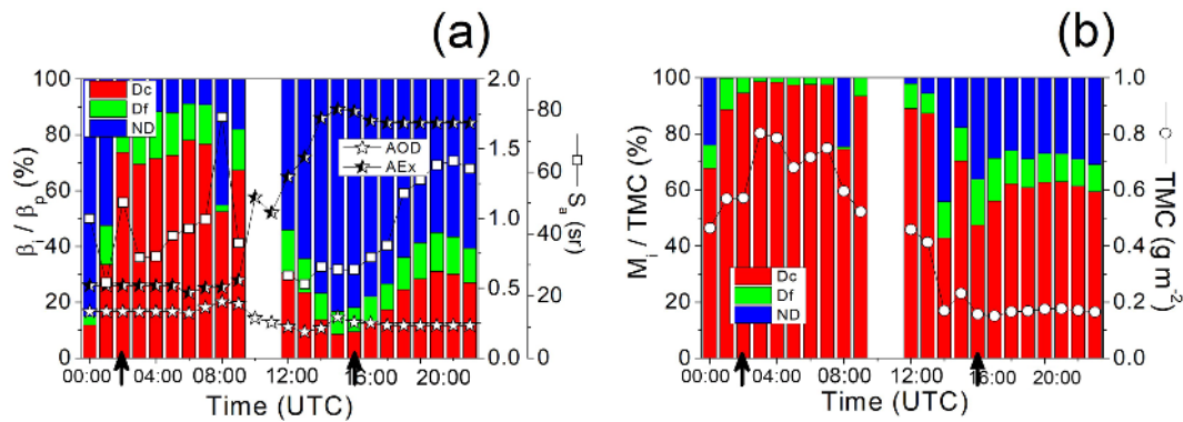
Figure 3. Dust event on 5 July 2016. Evolution of the relative contribution (a) \frac{\beta_i}{\beta_p} (%) and (b) \overline{M}_i / \text{TMC} (%) (the bar over the variable are removed in the figure for clarity) for each aerosol component throughout the day: Dc (red bars), Df (green bars) and ND (blue bars), which denote dust coarse, dust fine and non-dust aerosols. In (a) (right axis) AERONET hourly averaged AOD and AEx (white and black–white stars, respectively) and KF-derived S_a (lidar ratio, sr; square symbols) values are reported; in (b) (right axis) TMC (total mass loading, \text{g m}^{-2} ; open circles) is also included. Black arrows on the time axis indicate selected times for those vertical profiles shown in Fig. 4.
