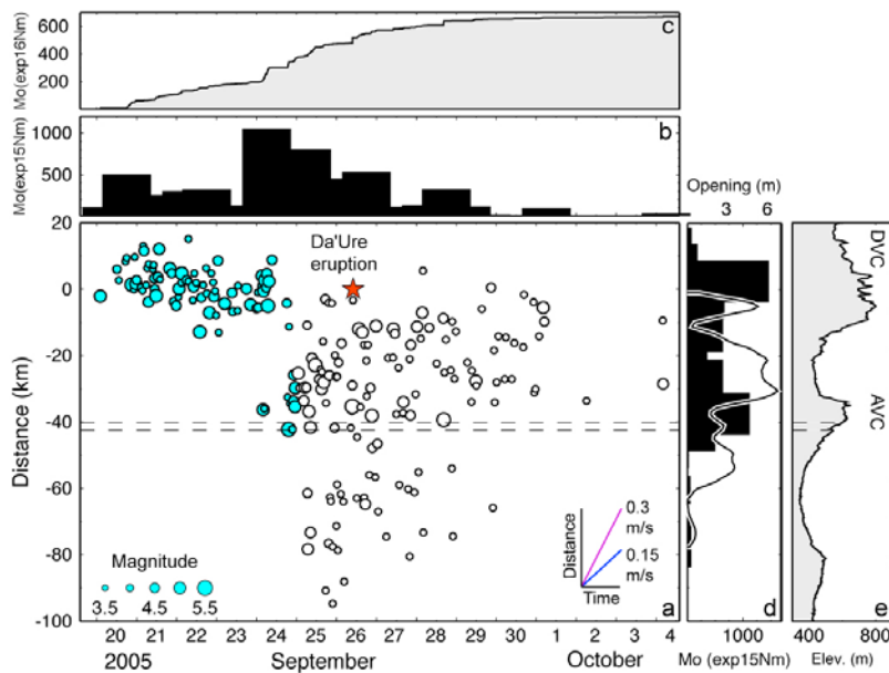
Figure 3. (a) Position of earthquakes along the Manda-Harraro rift plotted against event origin time, showing migration of seismic activity. Purple and blue lines in the bottom right corner illustrate migration velocities of 0.3 m/s and 0.15 m/s, respectively. Earthquake position is defined by projecting epicenters onto the plane of the dike. Earthquakes are colored as in Figure 1. Two parallel dashed lines define the estimated position of the dike source beneath AVC. (b) Histogram shows seismic moment release at 12 hour intervals. (c) Cumulative seismic moment release against time. (d) Black curve shows along-dike variation in horizontal opening modeled from InSAR data [Hamling et al. , 2009]. Histogram shows seismic moment release in 5-km intervals. (e) Along-rift topography. DVC is Dabbahu Volcanic Complex, and AVC is Ado' Ale Volcanic Complex. Red star shows the September 26, 2005 eruption site.
