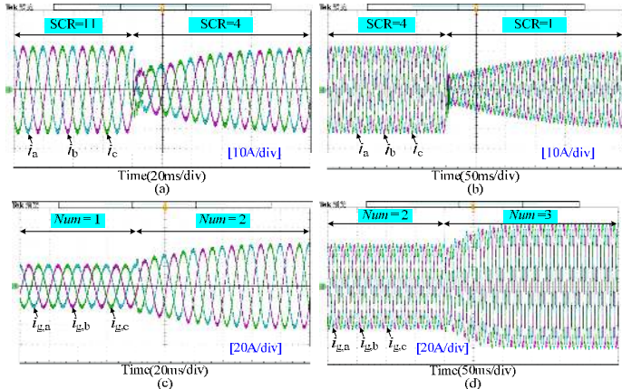
Fig. 10 Experimental results of VSG under different conditions. (a) SCR is decreased from 11 to 4; (b) SCR is decreased from 4 to 1; (c) Num is increased from 1 to 2; (d) Num is increased from 2 to 3.
