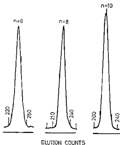
Figure 3. GPC of purified telomers.
