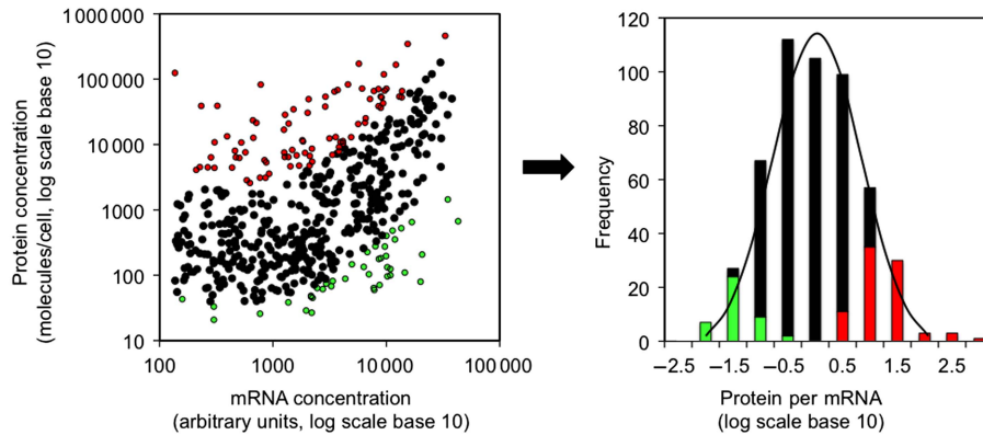
Figure 2 Human protein and mRNA concentrations. Left: protein and mRNA concentrations correlate significantly at a log–log scale ( N=512 , R^2=0.29 , R_s=0.46 with P -value < 2.2e-16 ). Right: genes with extremely high (red) or low (green) protein-per-mRNA ratios are likely regulated at the level of translation or protein stability. Source data is available for this figure at www.nature.com/msb .
