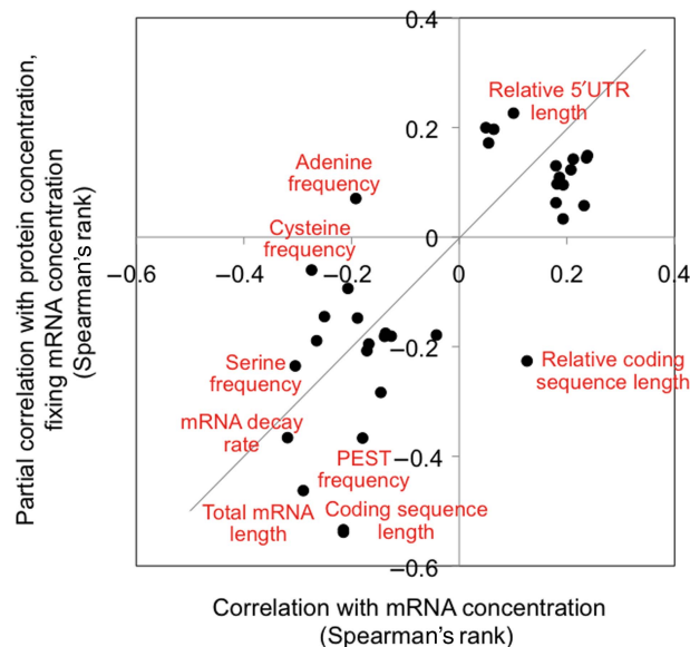
Figure 4 Concordance of mRNA and protein expression regulation. The figure shows the correlation coefficients for features listed in Table I. All correlations are listed in the Supplementary information; x axis: Spearman's rank correlation between the respective feature, and the mRNA concentration, which is the combined outcome of transcription and mRNA decay; y axis: partial Spearman's rank correlation between the respective feature and the protein concentration, fixing variation in mRNA concentration, which describes the combined outcome of translation and protein degradation.
