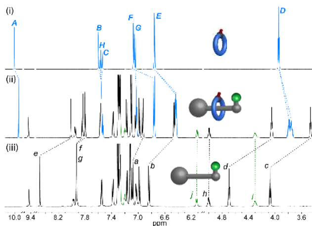
Figure 1. ^1\text{H} NMR spectra (600 MHz, d_6 -acetone, 298 K) of (i) macrocycle 2 , (ii) rotaxane 1 , (iii) free thread 5 . The assignments correspond to the lettering shown in Scheme 1.
