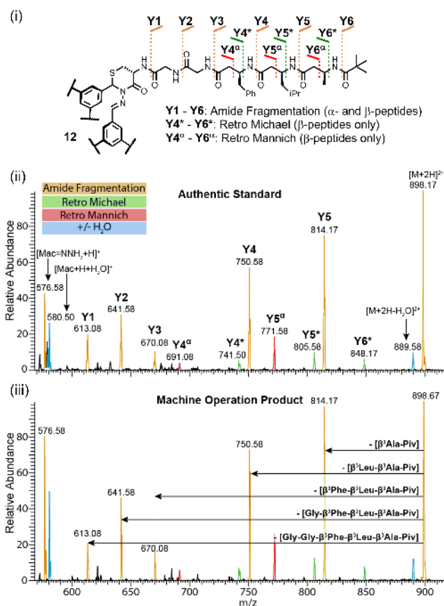
Figure 2. Tandem mass spectrometry sequencing of 12 . Anal-
