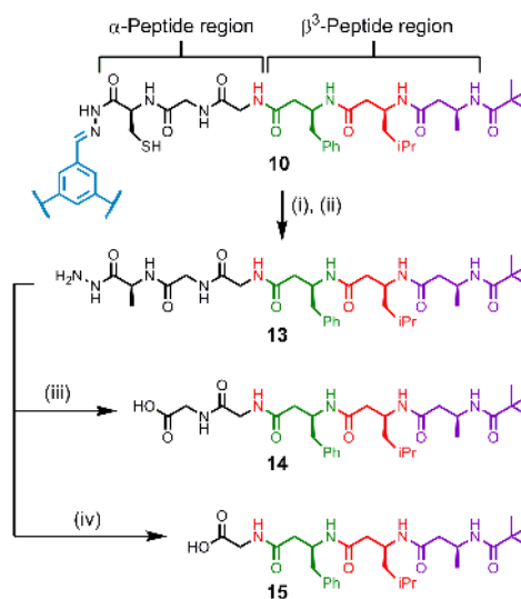
Scheme 3. Enzymatic Liberation of the \beta^3 -Peptide Region of the Machine Product from the NCL Catalyst Site. a
