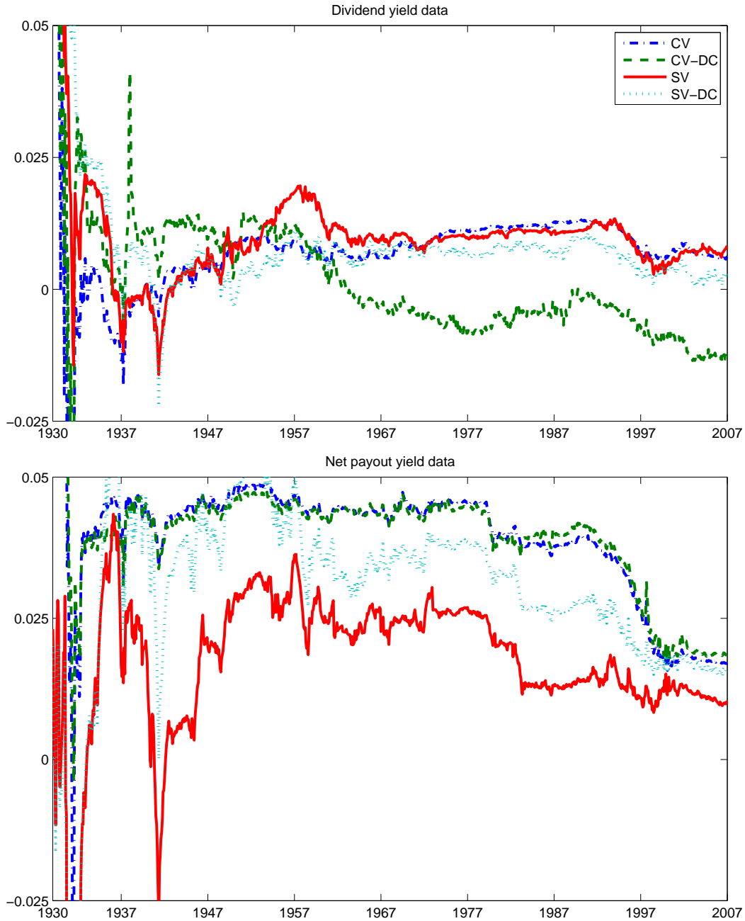
Figure 3: Predictability coefficient
