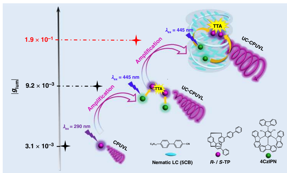
Fig. 1 The process of sequentially amplified CPUVL. Chemical structures of R / S -TP, 4CzIPN, 5CB and schematic representation of sequentially amplified CPUVL. R ( S )-TP showed a weak CPUVL emission ( |g_{\text{lum}}| = 3.1 \times 10^{-3} ) in toluene solution when excited by the 290 nm. After embedding with achiral sensitizer 4CzIPN, UC-CPUVL could be observed under the excitation of 445 nm continuous wave laser (A 445 nm short-pass filter was used). Due to the amplification effect photon upconversion on CPUVL emission, the g_{\text{lum}} value of UC-CPUVL reached to 9.2 \times 10^{-3} and showed three times larger than the downconversion process. Subsequently, chiral emitter and TADF sensitizer were adopted into the nematic liquid crystal (5CB), induced N*LC performed enhanced UC-CPUVL with a larger g_{\text{lum}} value ( |g_{\text{lum}}| = 1.9 \times 10^{-1} ), which could trigger the enantioselective polymerization of diacetylene with good stereoselectivity.
