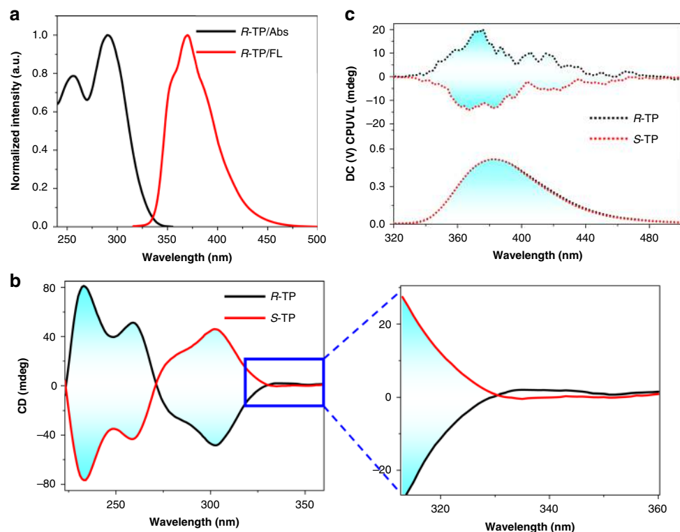
Fig. 2 CD and CPUVL spectra of R / S -TP in THF solution. a Normalized absorption and emission spectra of R -TP (0.01 mM, \lambda_{\text{ex}} = 290 nm) in THF solution. b CD spectra of R ( S )-TP in THF solution ( [R\text{-TP}] = [S\text{-TP}] = 0.01 mM). c CPL spectra of R ( S )-TP in THF solution ( [R\text{-TP}] = [S\text{-TP}] = 0.01 mM, \lambda_{\text{ex}} = 290 nm).
