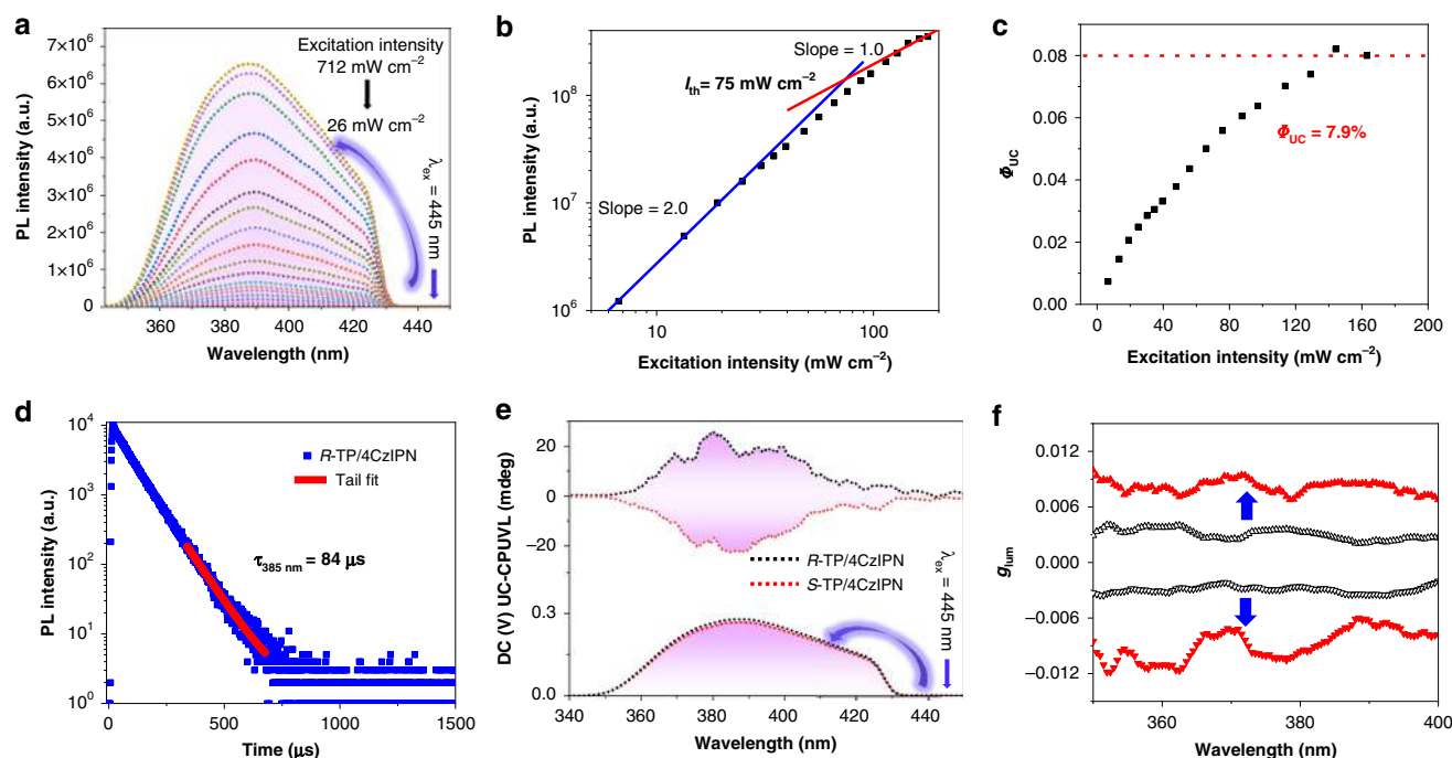
Fig. 3 Upconversion and UC-CPUVL process of R(S)-TP/4CzIPN in deaerated toluene solution. a Upconversion emission spectra of R-TP/4CzIPN with different incident excitation intensities of the 445 nm CW laser in deaerated toluene solution. b Double-logarithmic plots of the upconversion emission intensity of R-TP/4CzIPN in deaerated toluene solution as a function of the excitation intensity. c Upconversion efficiencies of R-TP/4CzIPN in deaerated toluene solution with different excitation light intensities of the 445 nm CW laser. d Time-resolved upconverted emission at 385 nm of the R-TP/4CzIPN in toluene solution ( \lambda_{\text{ex}} = 445 \text{ nm} ). e UC-CPUVL spectra of R-TP/4CzIPN and S-TP/4CzIPN in deaerated toluene solution ( \lambda_{\text{ex}} = 445 \text{ nm} ). f Luminescence dissymmetry factor g_{\text{lum}} of UC-CPUVL versus wavelength. R-TP/4CzIPN excited by 445 nm CW laser (red triangle); R-TP excited by 290 nm (white triangle); S-TP/4CzIPN excited by 445 nm CW laser (red inverted triangle); S-TP excited by 290 nm (white inverted triangle). ([R-TP] = [S-TP] = 3 mM, [4CzIPN] = 0.1 mM). For all the upconversion measurements, a 445 nm short-pass filter was used.
