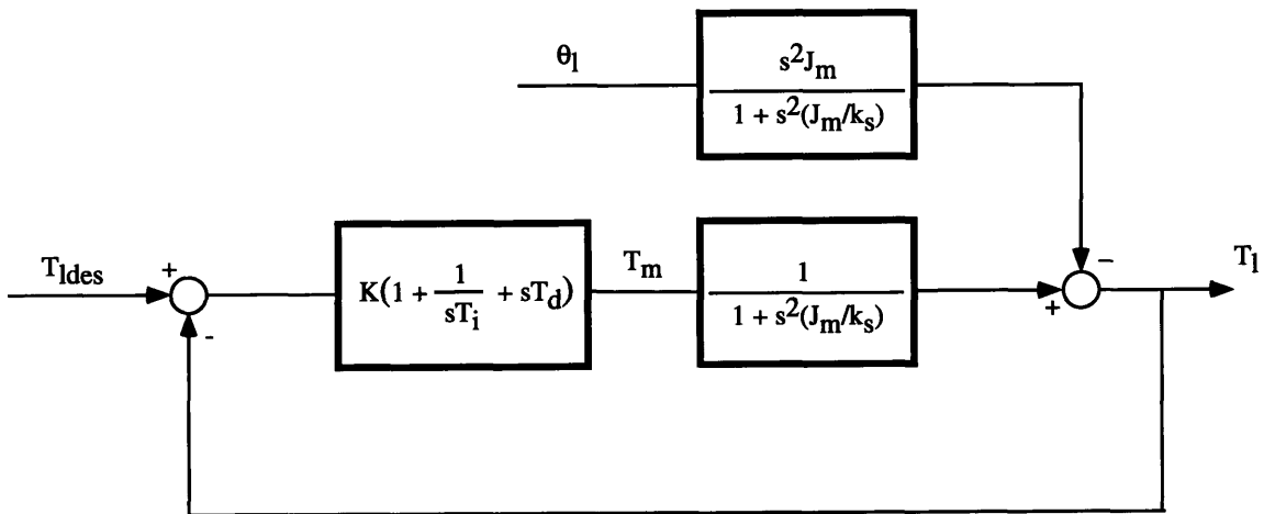
Figure 3-3: Closed loop system
