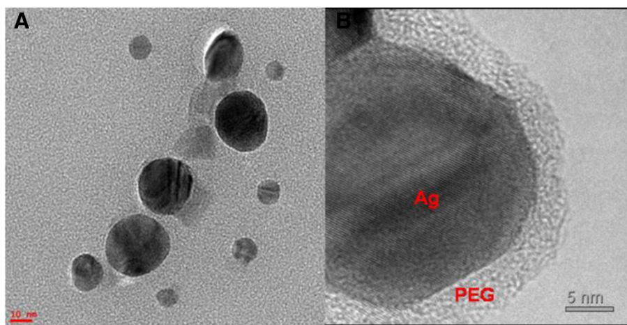
Figure 2 TEM characterization. (A) TEM images of PEG-reduced AgNPs obtained by rapidly adding AgNO 3 to the aqueous PEG solution. (B) Atomic-scale resolution TEM image of one PEG-reduced AgNP exhibiting the 5-nm PEG layer around the silver core. Spherical PEG-coated AgNPs of narrow size distribution are visible.
