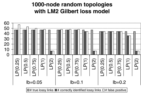
Fig. 11. Effects of different weights in LP: A LM_2 Gilbert loss model for 1000-node random topologies with maximum degree = 10 and f = 0.95 . We vary the loss threshold l_b , and only the links with loss rate higher than l_b are considered lossy.
