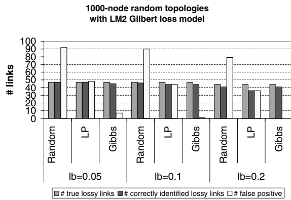
Fig. 9. A LM_2 Gilbert loss model for 1000-node random topologies with maximum degree = 10 and f = 0.95 . We vary the loss threshold l_b , and only the links with loss rate higher than l_b are considered lossy.
