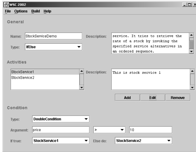
Figure 12: The main window of Service-Com.
