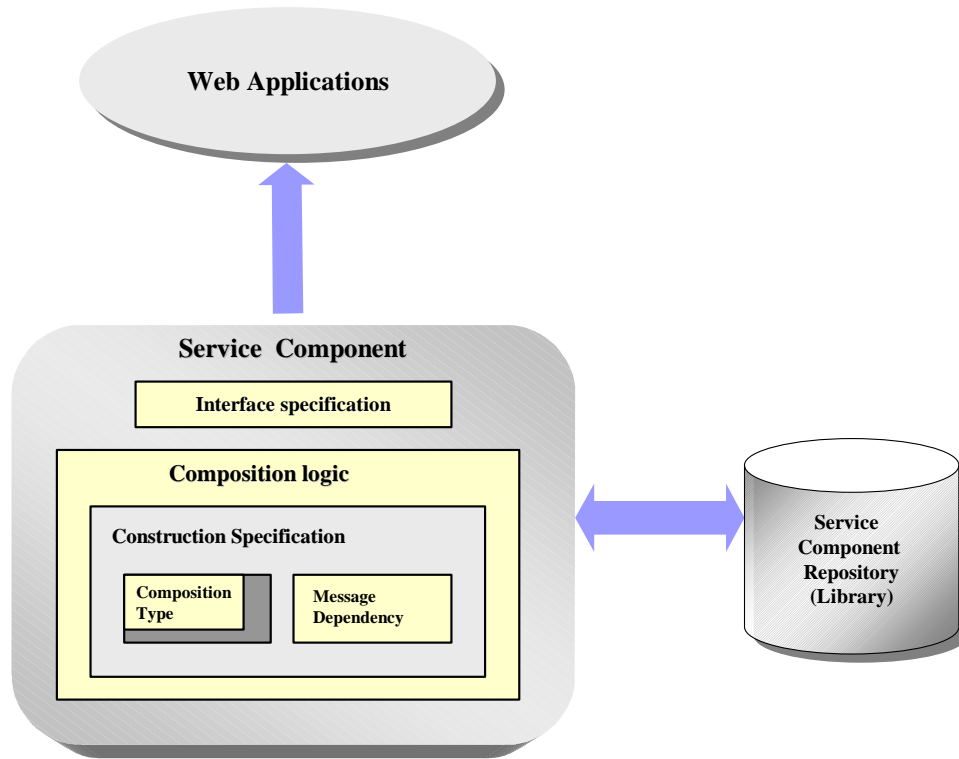
Figure 3: Service component ingredients.
