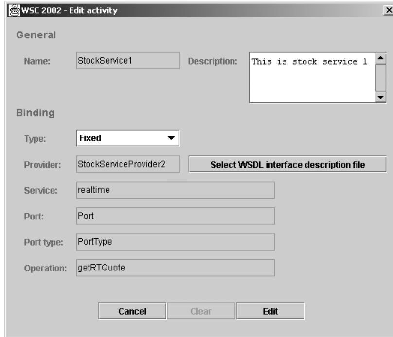
Figure 13: The activity dialogue window for a fixed binding
