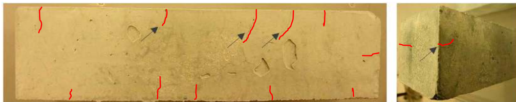
Figure 16. Visual observations of sample S100 surfaces. Samples were cured for 14 days (fog room, at 20\text{ }^\circ\text{C} and 99% RH) and subsequently removed to laboratory conditions, at 20\text{ }^\circ\text{C} and 55% RH. Arrows point to microcracks patterns, which are coloured in red. (The microcracks were most present on the top surface, while on the other sides of samples their appearance was less).
