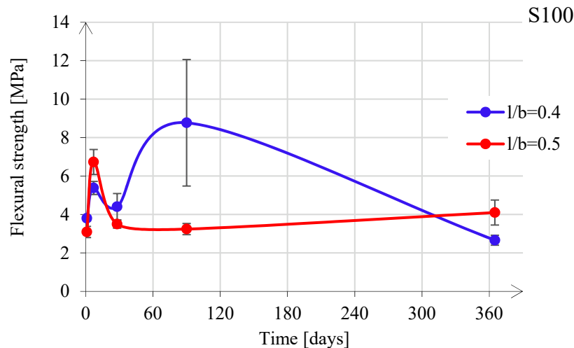
Figure 13. Flexural strength development for S100 paste.
