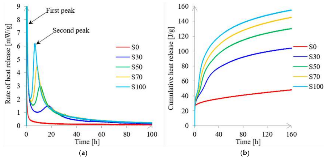
Figure 9. Calorimetric curves for the rate of heat release (a) and cumulative heat release (b) for alkali-activated pastes with l/b = 0.5 .
