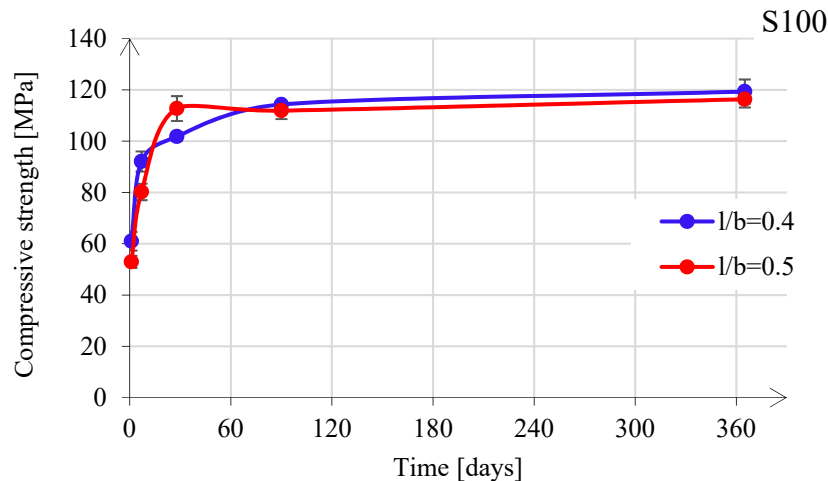
Figure 10. Compressive strength development for S100 paste.
