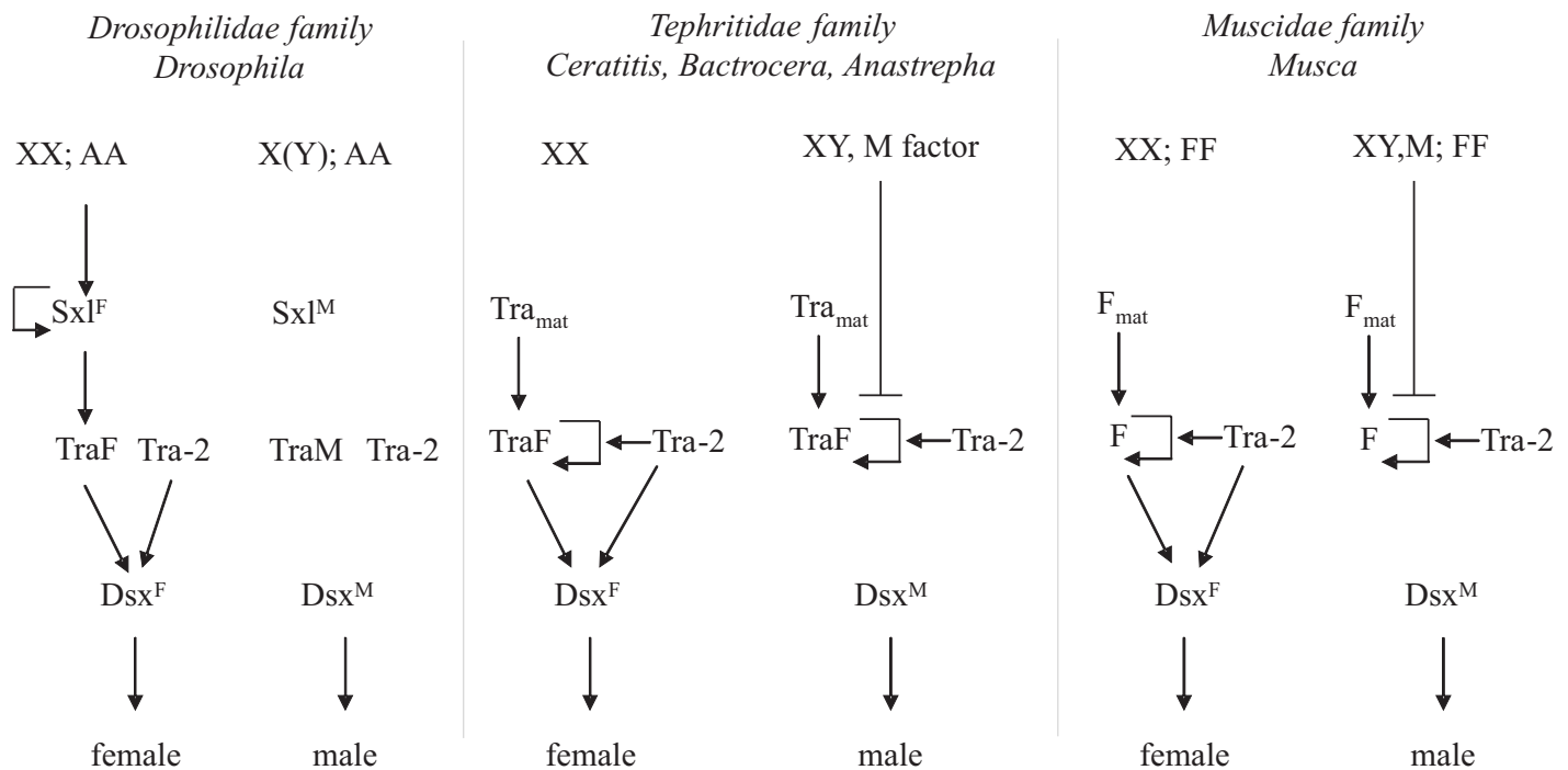
Fig. 9. The sex determination gene cascade in Drosophila , Ceratitis , Bactrocera , Anastrepha and Musca . Tra_{mat} and F_{mat} indicate maternal Tra and F product respectively. The production of Dsx^M protein is the default state. The scheme for the Tephritidae is modified from Pane et al. (2002), and that for the Muscidae from Burghardt et al. (2005).
