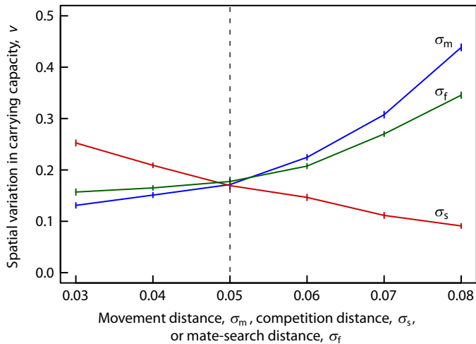
Figure S6 | Minimum level of spatial variation \nu in local carrying capacity needed to ensure long-term coexistence in a two-dimensional bimodal landscape. The spatial variation \nu is increased until the average persistence time of mating types in 20 replicate runs exceeded 10K generations (vertical lines indicate standard errors). The three curves show the effects of the width \sigma_s of the competition distribution (red), the width \sigma_f of the mate-search distribution (green), and the width \sigma_m of the movement distribution (blue), while holding all other parameters constant at their values in Fig. 1d. In the other figures, the following values (indicated by the vertical dashed line) are used: \sigma_s = 0.05 , \sigma_f = 0.05 , \sigma_m = 0.05 .
