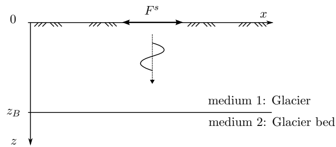
Figure 1. Schematic representation of the seismic shear wave traveling downwards in a two-layer one-dimensional system. Medium 1 represents the ice body (assumed as an elastic medium) and medium 2 is the porous basement (assumed as a poroelastic medium)
