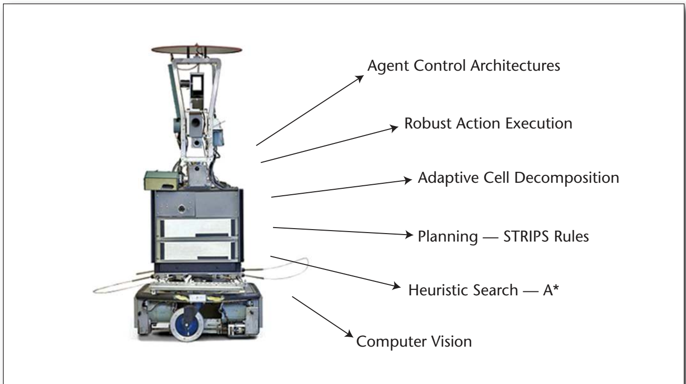
Figure 11. Shakey's Achievements.
