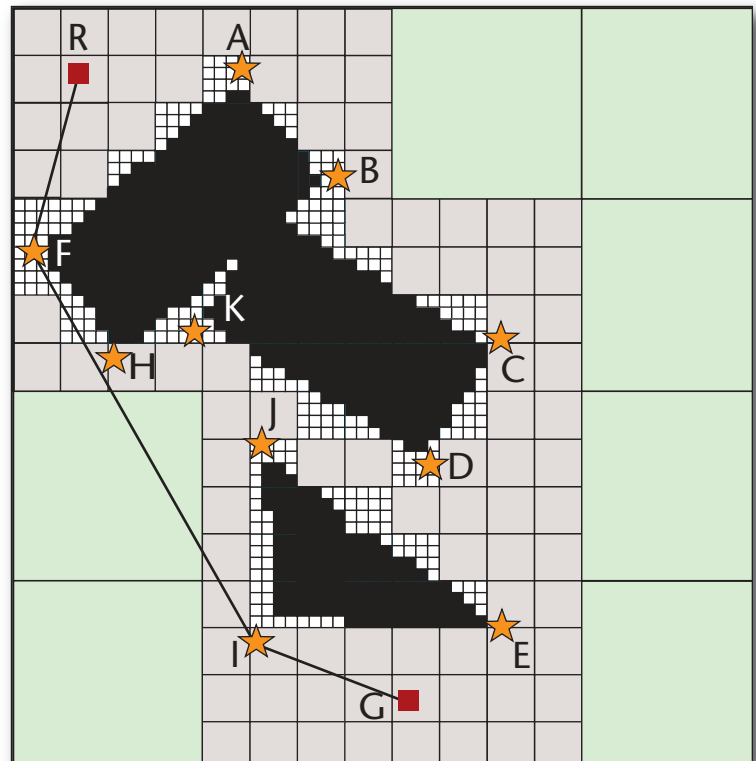
Figure 13. Shakey's Adaptive Grid Model.
