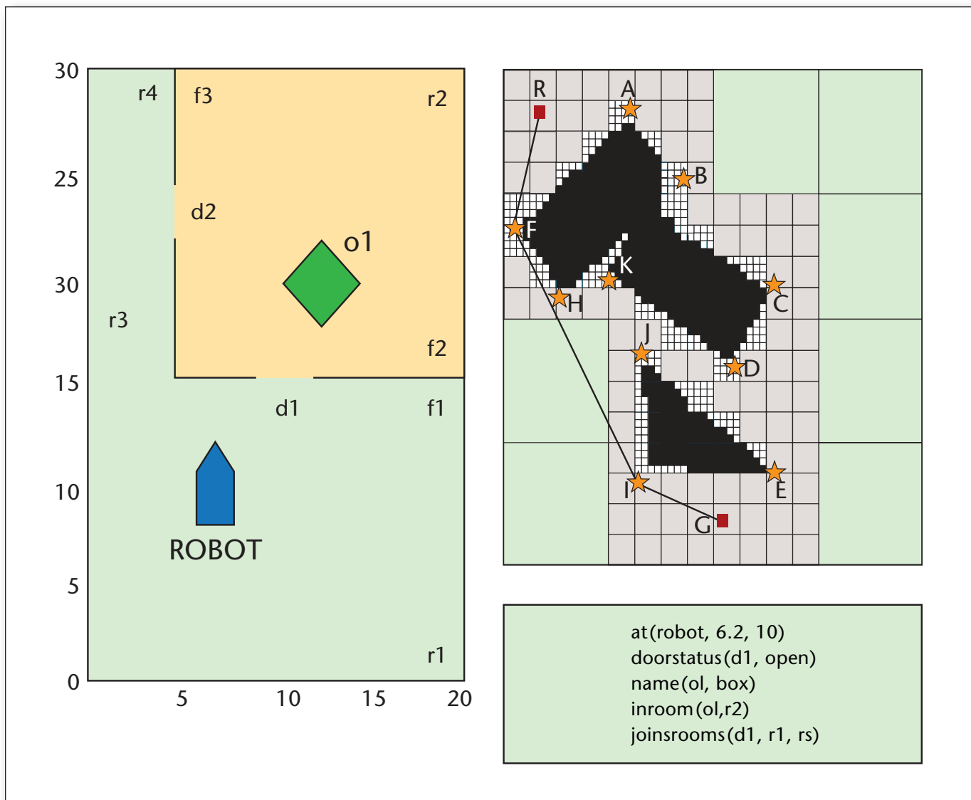
Figure 4. Predicate Calculus Model Fragment with Plan View of World and Grid Model
