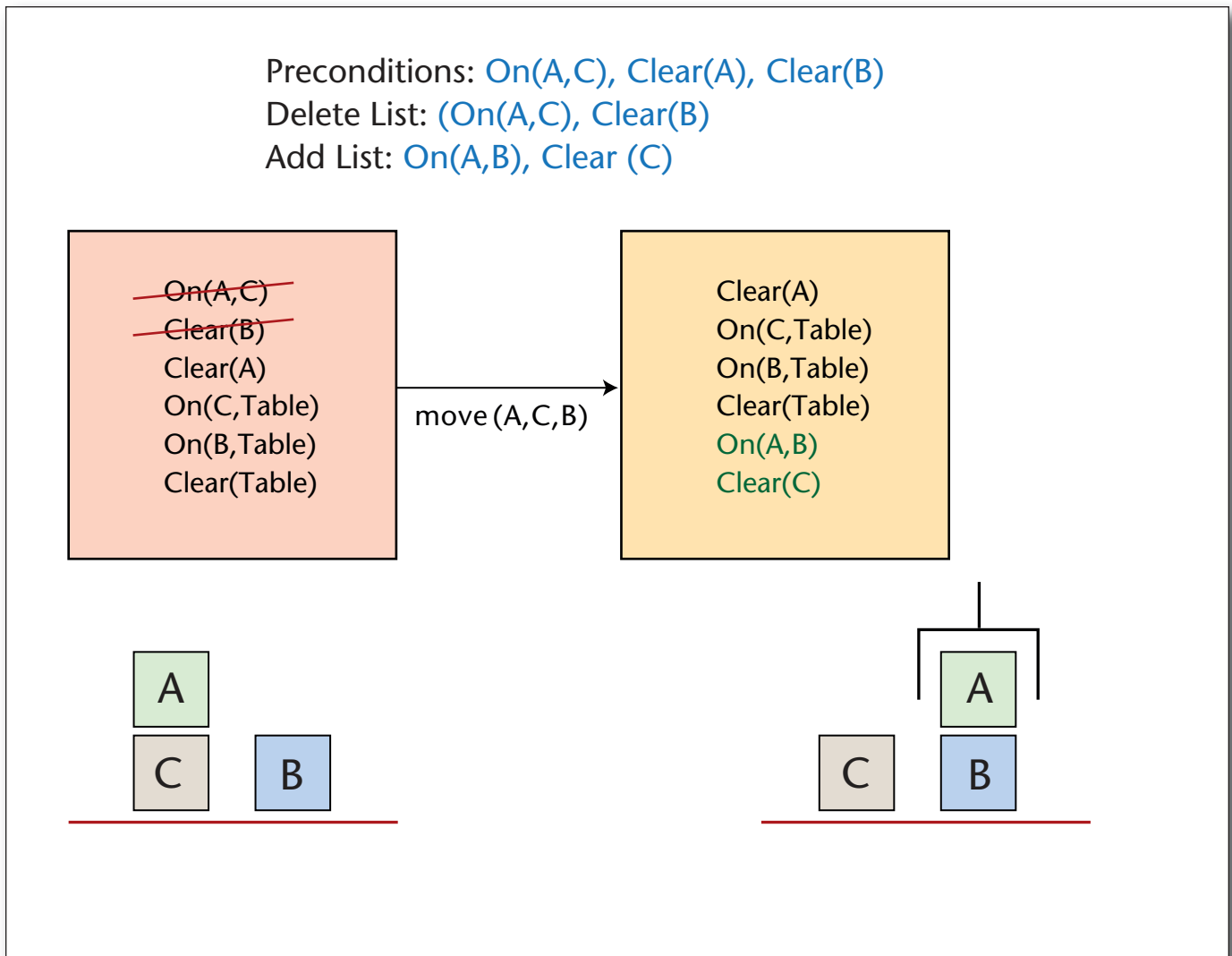
Figure 14. Application of a STRIPS Rule.
