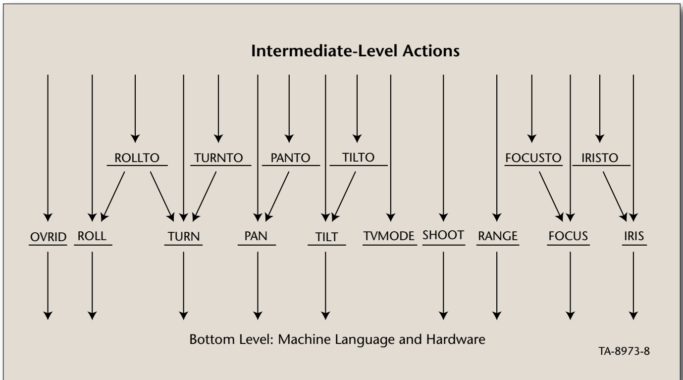
Figure 6. Low-Level Actions.
