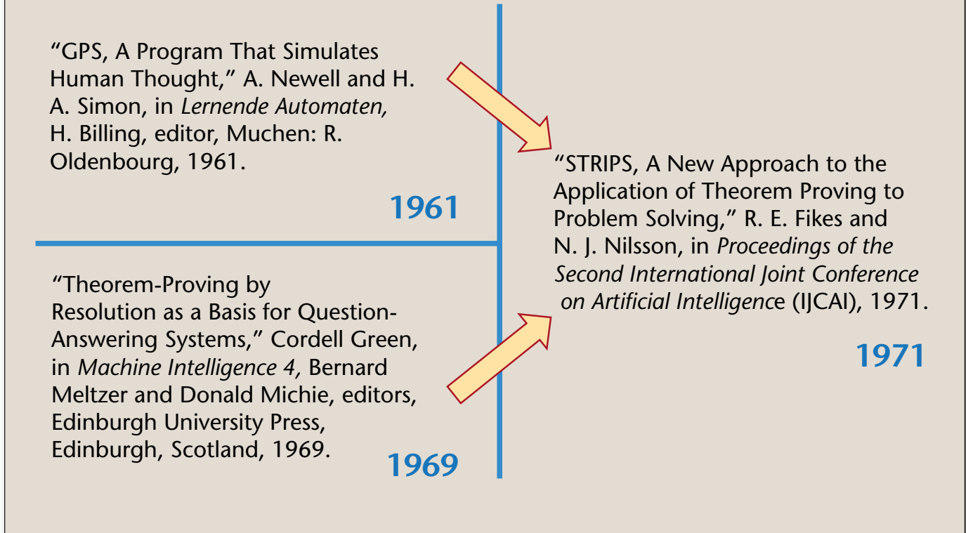
Figure 8. STRIPS.
