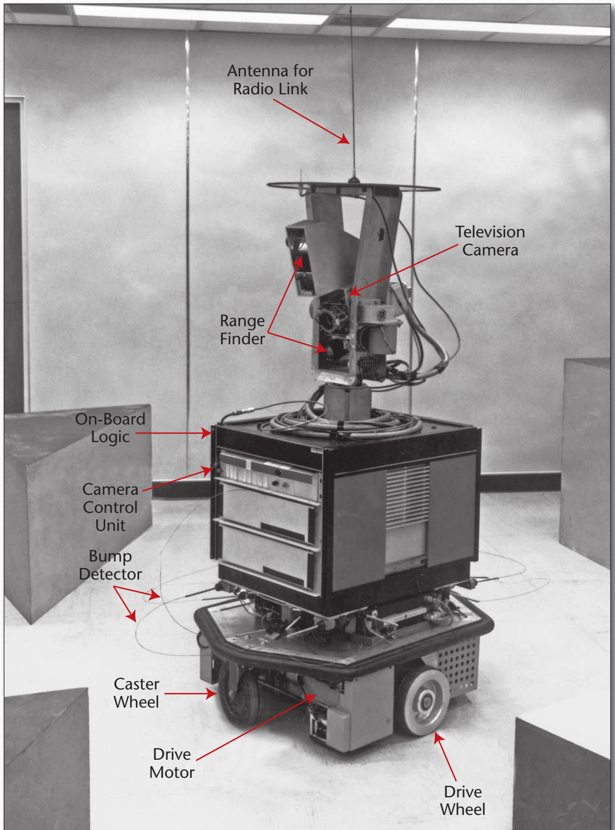
Figure 2. Shakey with Components Labeled.
