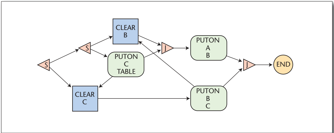
Figure 15. A Hierarchical Task Network.
