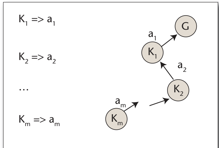
Figure 12. Teleo-Reactive Programs.
