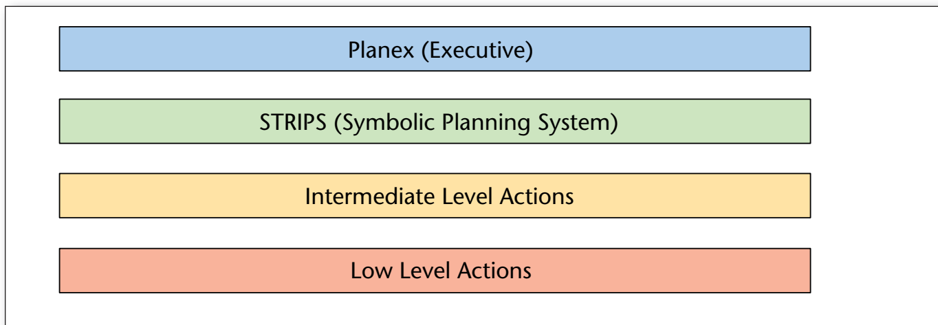
Figure 5. Layered Software Architecture.
