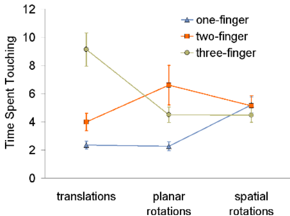
Figure 11. There was a significant interaction between technique and movement type. For the one-touch technique, participants performed more spatial rotations than translations or planar rotations and for the three-touch technique, participants spent more time performing translations than planar or spatial rotations. The difference in movement type did not differ significantly for the two-touch technique.
