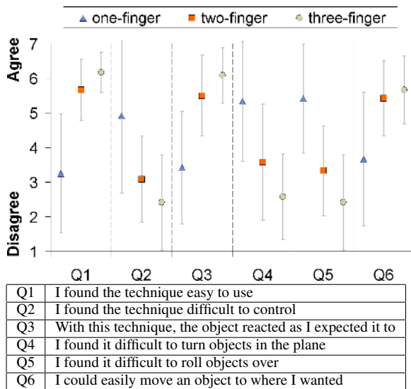
Figure 13. Mean ratings and (standard deviations) on the follow-up questionnaire. Users rated their level of agreement on a scale from 1 (strongly disagree) to 7 (strongly agree).
