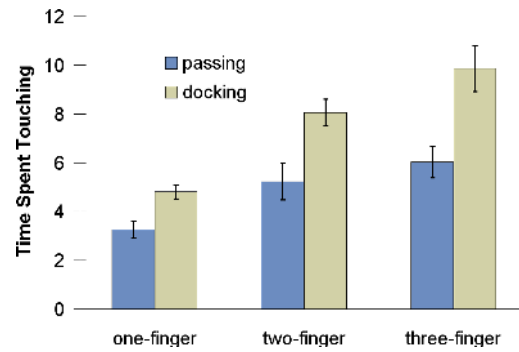
Figure 10. Mean time spent touching the object, separated into translations, planar rotations and spatial rotations.
