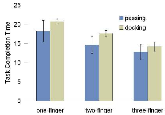
Figure 8. Mean TCTs for both the passing task and the docking task. In both cases, three-touch interaction is fastest, followed by two-touch, and one-touch is slowest.
