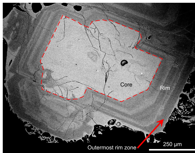
Figure 5. Back scattered electron images of a representative plagioclase phenocryst from the 1914 Plinian pumice. The plagioclase has a calcic core and a thick (~200 \mu\text{m} ) relatively sodic rim with oscillatory zoning. The outermost homogeneous zone with a thickness of >10 \mu\text{m} (typically 20–30 \mu\text{m} ) was analysed for the hygrometer calculation.
