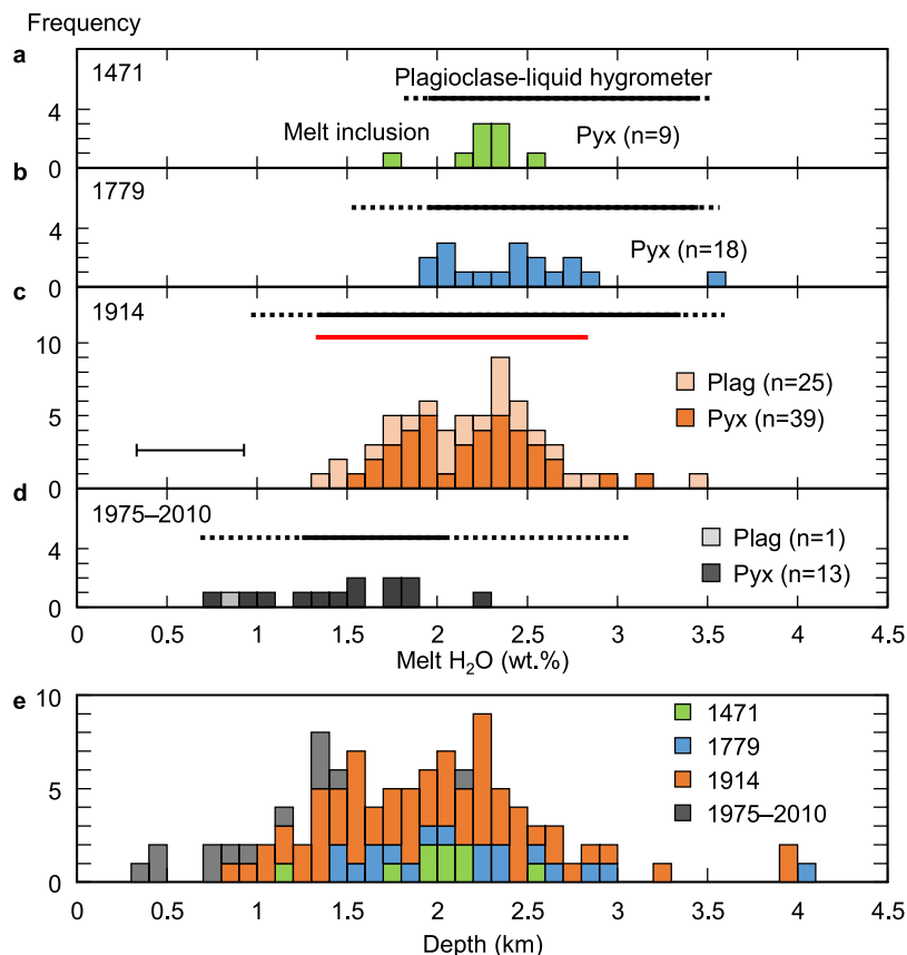
Figure 4. Frequency distribution of melt inclusion H_2O contents and estimated depths. H_2O contents in melt inclusions from the Plinian eruptions in 1471 (a), 1779 (b), and 1914 (c), and Vulcanian explosions in 1975–2010 (d) measured by FT-IR reflectance spectroscopy. Black and red bars represent the melt H_2O contents calculated with a plagioclase-melt hygrometer 33 . See Supplementary Fig. S3 for details. The analytical accuracy of the FTIR analysis is shown in c. (e) Magma storage depths estimated from the final equilibrated pressure of H_2O contents in melt inclusions calculated with the H_2O solubility model 32 .
