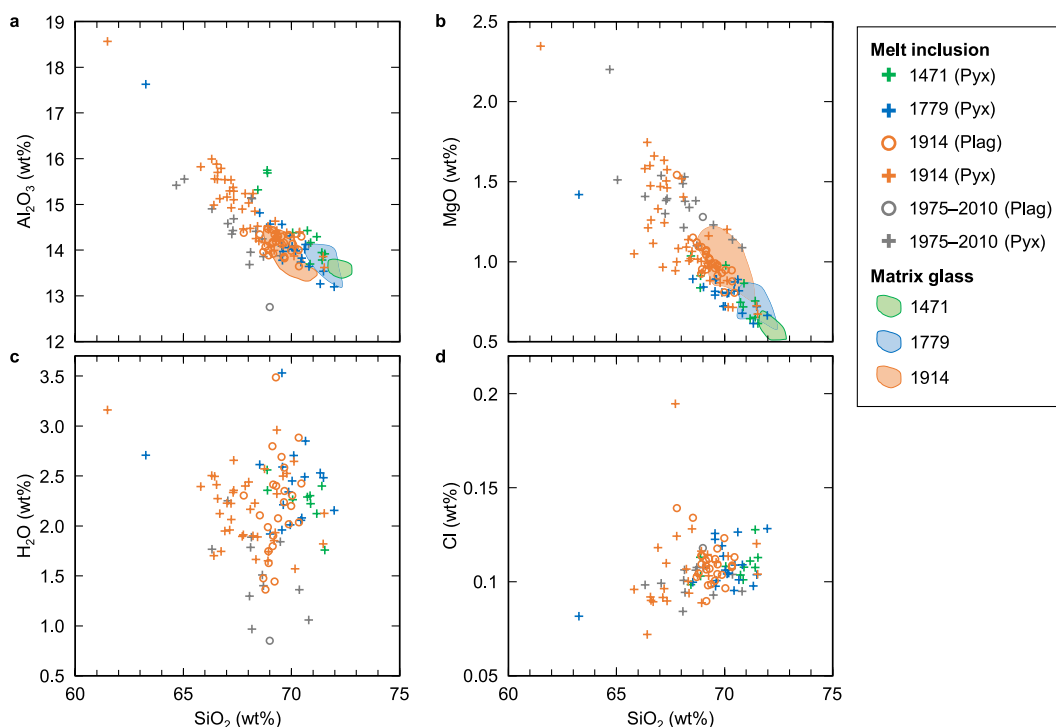
Figure 3. SiO 2 variation diagrams of melt inclusion compositions. The major element composition (a: Al 2 O 3 , b: MgO) of the most silica-rich inclusions coincides with that of matrix groundmass matrix glass for each Plinian eruption. (c) H 2 O contents do not exhibit a systematic correlation with SiO 2 contents. (d) Cl contents of melt inclusions in plagioclase (Plag) do not correlate with SiO 2 contents, whereas those in pyroxene (Pyx) have a weak negative correlation.
