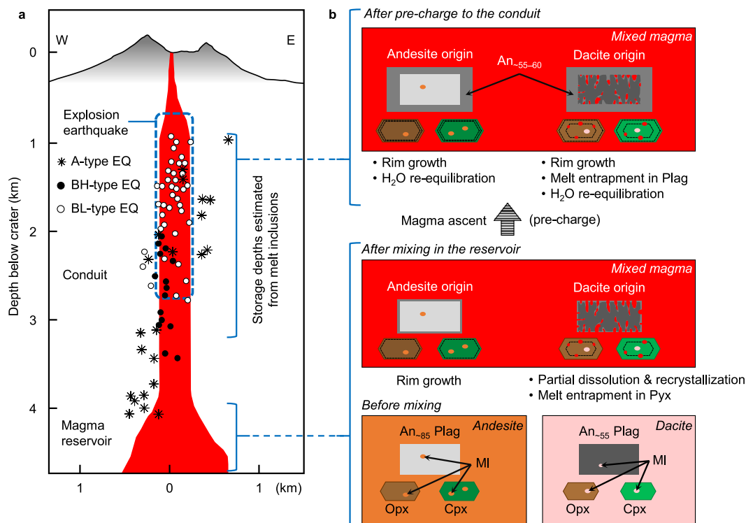
Figure 6. Magma pre-charge processes recorded in phenocryst microstructures in the historic Plinian eruptions. (a) Hypocentre distribution of volcanic earthquakes of recent Vulcanian eruptions 12 that coincides with the final magma storage depths of the historic Plinian eruptions. A-type earthquakes (EQ), and BL- and BH-types are caused by brittle fracture of rocks and fluid movement, respectively 11 . (b) Pyroxene-hosted melt inclusions, trapped at various timings, were re-equilibrated after pre-charge to the conduit. Melt channels in plagioclase formed by partial dissolution upon magma mixing were enclosed in the conduit as melt inclusions. See Supplementary Information for details of mixing endmembers.
