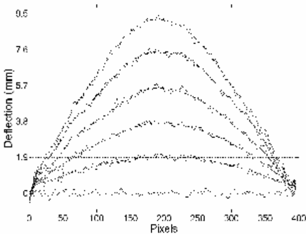
Figure 3: Deflection measurement results.
