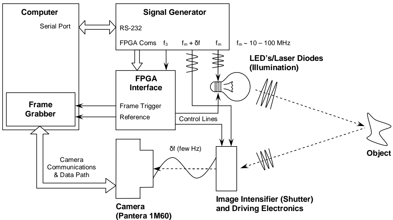
Figure 1: Block diagram of current range imaging hardware including signal and dataflow.
