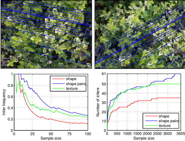
Figure 9. Scene with leaves. For this kind of scene, the use of shape pairs is advantageous.
