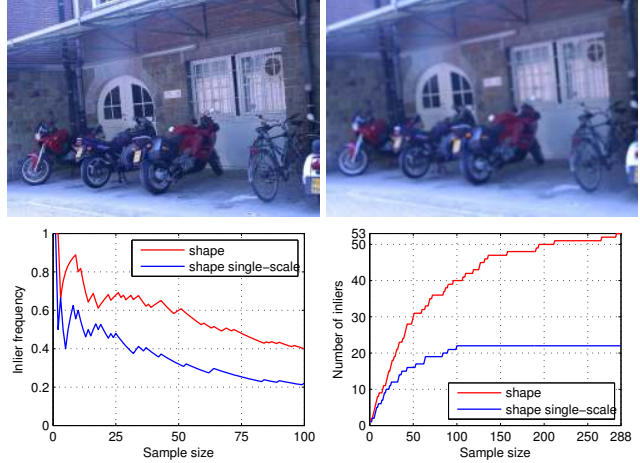
Figure 11. A scene with de-focus blur. The multi-resolution MSER provides better performance than using only the original resolution.
