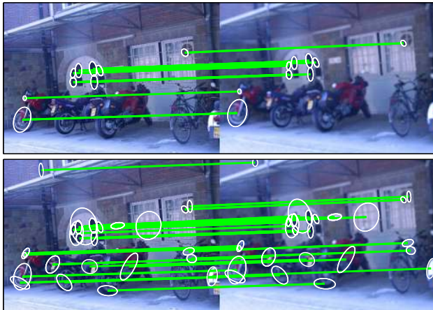
Figure 13. Correspondences found on de-focus blur scene. Top image shows the 22 correspondences found using single resolution MSERs. Bottom image shows the 53 correspondences found using multi-resolution MSERs.
