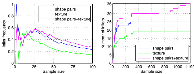
Figure 17. Combination of shape pair and texture patch features for the day and night pair in figure 16.
