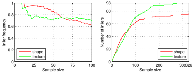
Figure 5. Performance of shape and texture descriptors on the scene in figure 3.
