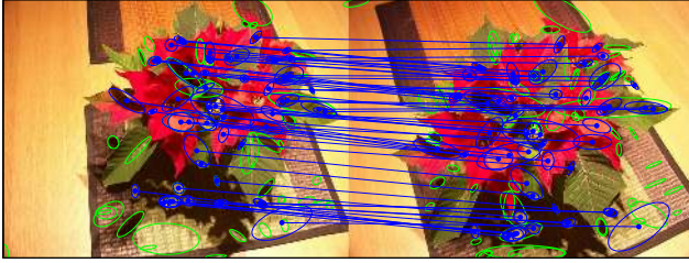
Figure 4. The 56 accepted correspondences are shown in blue. Features from rejected correspondences are shown in green. (Using MSER area threshold 100 pixels, instead of 30, for clarity of presentation.)
