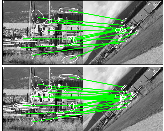
Figure 14. Correspondences found on scale change scene. Top image shows the 22 correspondences found using single resolution MSERs. Bottom image shows the 33 correspondences found using multi-resolution MSERs.
