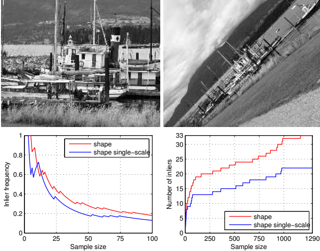
Figure 12. A scene with scale change. Again, the multi-resolution MSER gives better performance.
