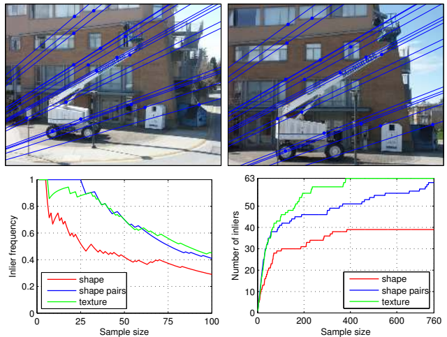
Figure 15. Crane scene, with and without pairs.
