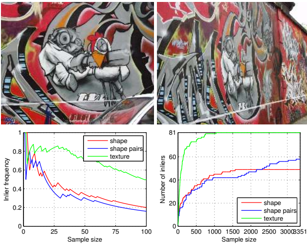
Figure 10. A planar scene with view change. In this case, the texture descriptor has better performance than the shape descriptor.
