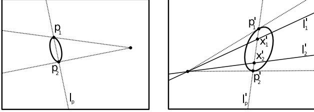
Figure 2. Epipolar geometry. Left: Construction of tangency points \mathbf{p}_1 and \mathbf{p}_2 from the polar line l_p . Right: Induced epipolar tangents l'_1 and l'_2 , and the tangency points in this view. The intersection points \mathbf{x}'_1 and \mathbf{x}'_2 are used to compute the overlap error.
