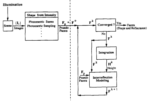
Figure 5: The shape and reflectance recovery algorithm.
