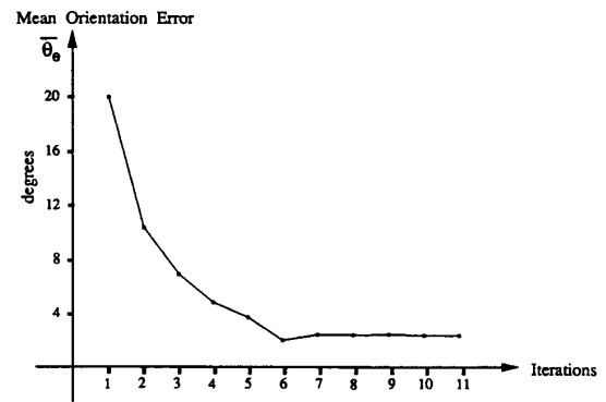
Figure 12: Convergence graph for the inverted pyramid shown in Figure 10.
