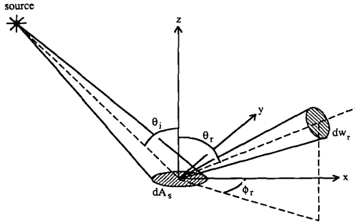
Figure 13: Basic geometry used to define radiometric terms.
