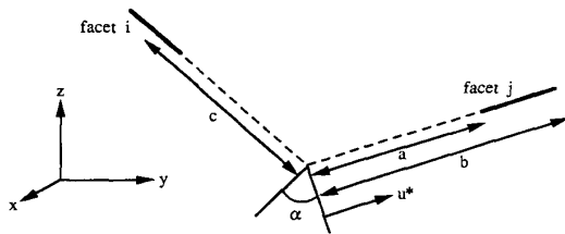
Figure 14: Cross-sectional view of two planar facets that are infinite in the x direction.
