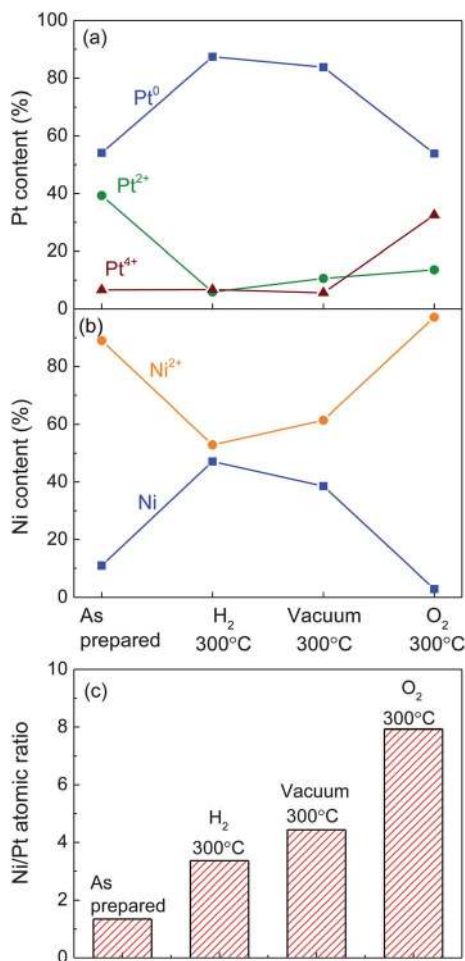
Fig. 6 Relative content of (a) Pt and (b) Ni species extracted from the XPS measurements in Fig. 5. (c) Ni/Pt atomic ratio obtained for the as prepared sample and analogous fresh samples after the indicated sample treatments.
