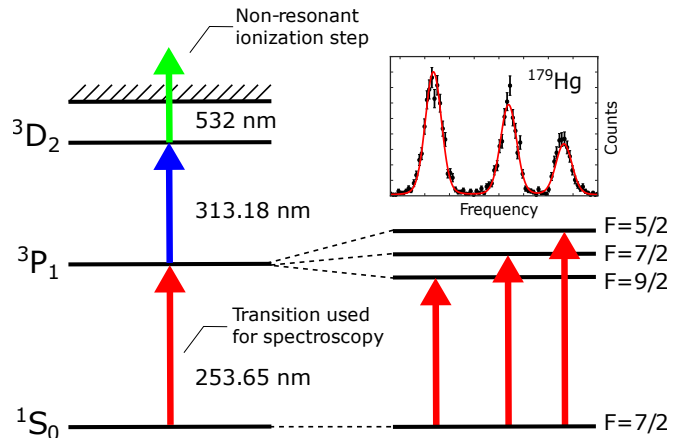
FIG. 3. Ionization scheme for mercury developed in [31], using the same transition for spectroscopy as in [1] and [33]. The right-hand side shows the splitting of the ^3P_1 level states with different total angular momentum F = I + J for an I = 7/2 nuclear spin with a corresponding exemplary HFS spectrum of ^{179}\text{Hg} . Energies and level splitting are not displayed to scale.
