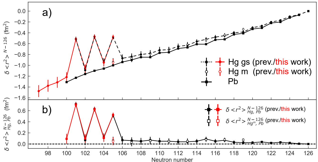
FIG. 9. a) Comparison of the change in mean-square charge radius for mercury and lead isotopic chains as a function of neutron number N , using N = 126 as a reference.
