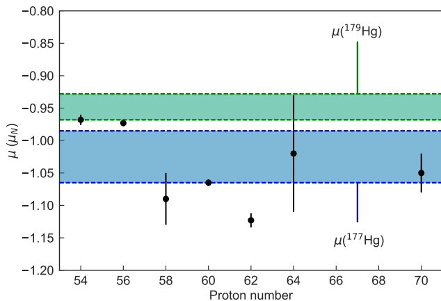
FIG. 10. Comparison of magnetic moments for N = 83 isotones, having one neutron in the ( \nu f_{7/2} ) shell above the closed shell N = 82 , with the measured \mu(^{177}\text{Hg}) and \mu(^{179}\text{Hg}) indicated by shaded boxes. Data from [65], [67] and references therein.
