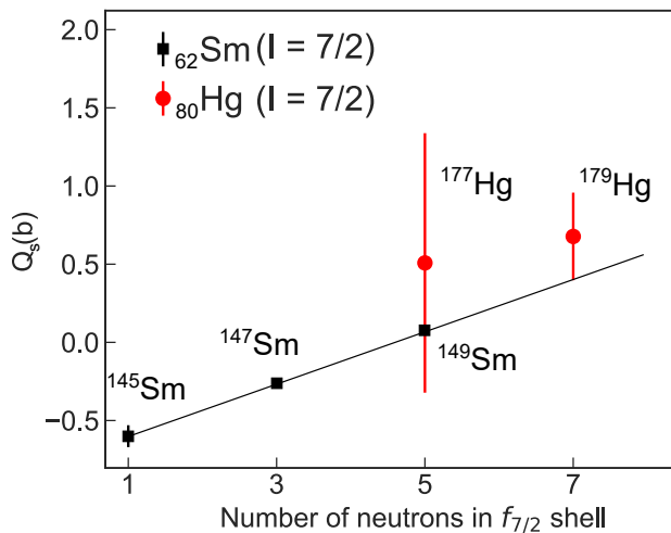
FIG. 11. Comparison of quadrupole moments for the ^{145,147,149}\text{Sm} isotopes (data from [65]), with measured values for ^{177,179}\text{Hg} corrected for the difference in charge radius between samarium and mercury.
