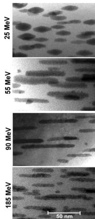
FIG. 7. TEM micrographs of 14.5 nm Pt NPs (prior to SHII) irradiated with 2 \times 10^{14} \text{ cm}^{-2} at different energies (as shown in each panel).
