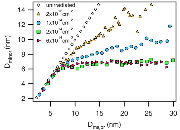
FIG. 3. (Color online) NP D_{\text{major}} versus D_{\text{minor}} according to SHII fluence, as determined from TEM.
