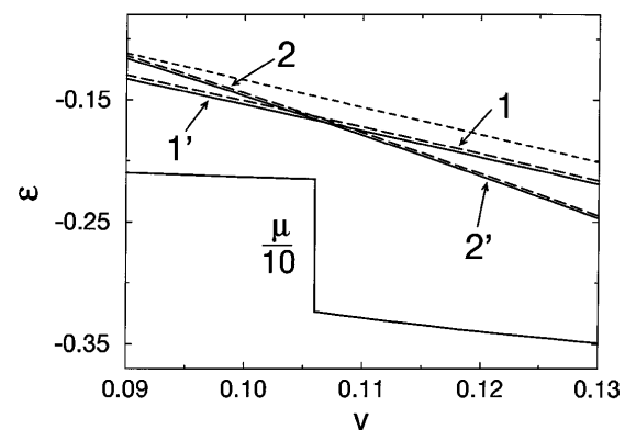
FIG. 4. Dimensionless island energy vs volume for r = 0.2 and \Gamma_2 > 0 . Solid lines correspond to equilibrium islands (1' and 2'). Adjacent long-dashed lines represent islands constrained to have no top facet (1 and 2). Upper dashed line corresponds to saddle point energy; see text. The bottom solid curve represents the dimensionless chemical potential \mu (divided by 10 to fit on graph). At the shape transition, \mu is discontinuous, which radically affects growth and coarsening.
