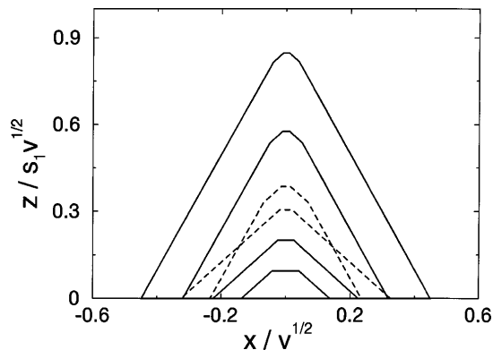
FIG. 2. Minimum-energy island shapes at different volumes, for s = 2, r = 0.2 , and \Gamma_2 > 0 . The volumes shown are v = 0.017 (the smallest size at which an island occurs in equilibrium), 0.05, 0.105 (two dashed islands), 0.2, and 0.4. The two dashed islands show the (energetically degenerate) shapes just before and after the shape transition at v = 0.105 .
