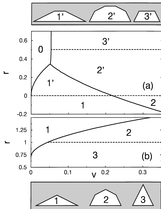
FIG. 3. Phase diagram (in two parts) showing island type vs volume v and surface energy parameter r . Six distinct island shapes occur, having the following: (1) shallow facet only; (2) shallow and steep facets; (3) steep facet only; (1') shallow and top; (2') shallow, steep, and top; and (3') steep and top. Phase (0) corresponds to the uniform flat film. The two cases are (a) \Gamma_2 > 0 , and (b) \Gamma_2 < 0 . Solid curves describe first-order phase transitions, while the horizontal dashed lines are second order.
