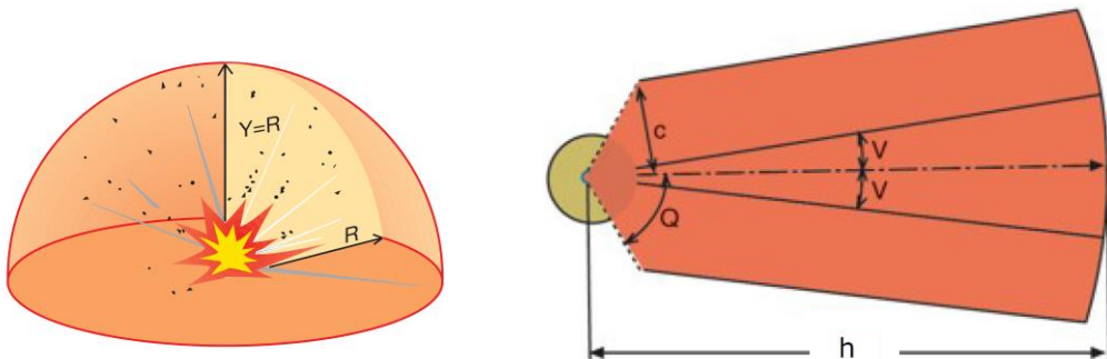
Figure 1. Hazardous area at explosion (left) and for shaped charge effects (right). (SwAF 2004 [2])
