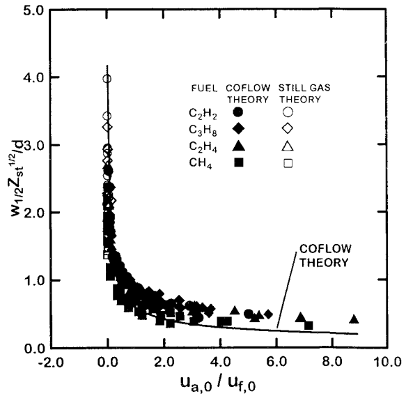
Fig. 5. Measured and predicted flame-sheet diameters as a function of air/fuel velocity ratios (large air/fuel velocity ratio limit).
