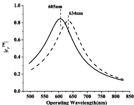
FIG. 6. The dispersion property of c_l^{\text{TM}} for a single concentric particle of outer radius 62 nm, with core made of \text{SiO}_2 and shell made of silver. The radii ratio is 0.851 for the dashed line, and 0.834 for the solid line. Silver follows a Drude model in this calculation.
