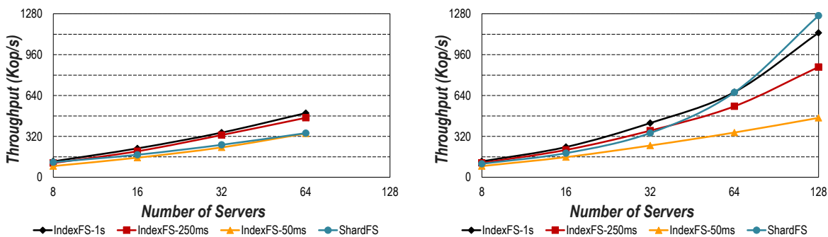
Figure 7: Aggregated throughput replaying an one-day trace collected from LinkedIn versus number of machines using either strong scaling (Section 4.2) or weak scaling (Section 4.3). Figure 7(a) on the left. Figure 7(b) on the right.
