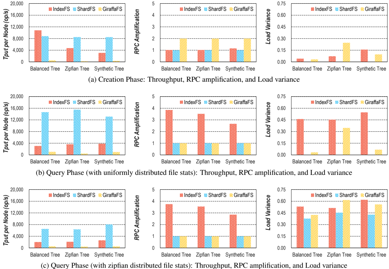
Figure 6: Performance comparison among IndexFS, ShardFS, and Giraffa creating and stating zero-byte files with 64 server machines and 64 client machines.
