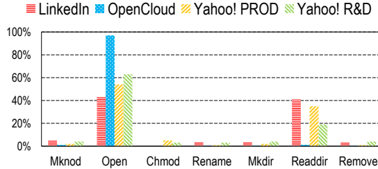
Figure 2: Distribution of file system operations in LinkedIn, Yahoo!, and OpenCloud traces.
