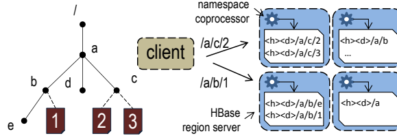
Figure 4: Giraffa stores its metadata in HBase, which partitions its table as a B-Tree. Each file or directory is mapped to an unique row at one HBase region server. The current implementation of Giraffa does not have hierarchical permission checking so no pathname resolution is performed.
