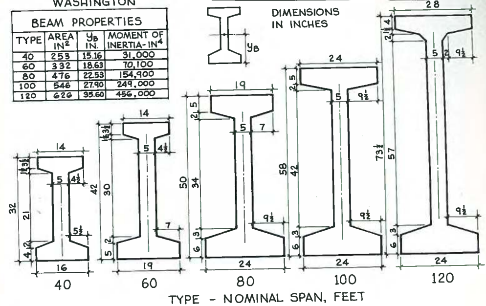
Fig. 75. Washington State standard beams.
