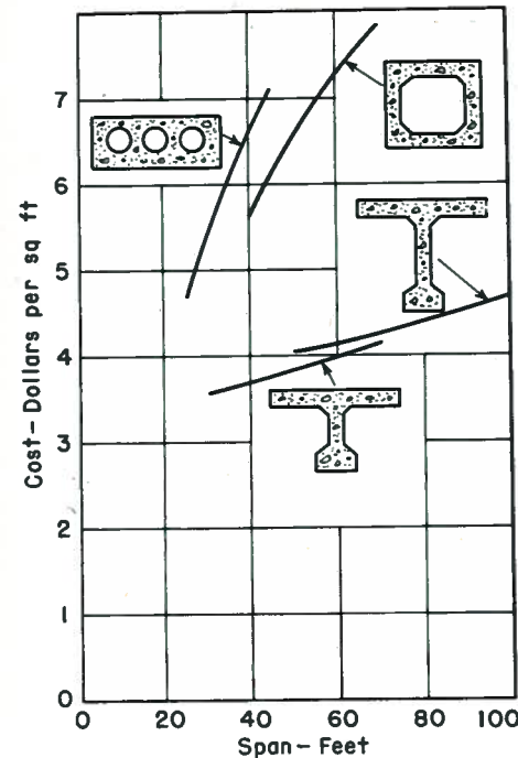
Fig. 71. Cost-span comparison of various bridge sections.
