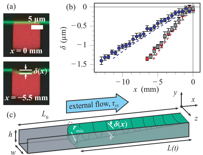
FIG. 2. (a) Representative groove cross-sections from the steady-state configuration of an experiment conducted at Q = 2 \text{ mL/min} with low viscosity oil, taken at the outlet slot ( x = 0 \text{ mm} ) and the far upstream end of the wetted groove ( x = -5.5 \text{ mm} ). (b) The steady-state deflection at the center of the groove, \delta(x) , with theoretical predictions (Supplemental Material) plotted as dashed lines. Gray is low viscosity oil at Q = 2 \text{ mL/min} , red is high viscosity oil at the same flow rate, and blue is low viscosity oil at Q = 1 \text{ mL/min} . (c) Schematic of one groove, showing geometric parameters and the shape of the interface deduced from (b).
