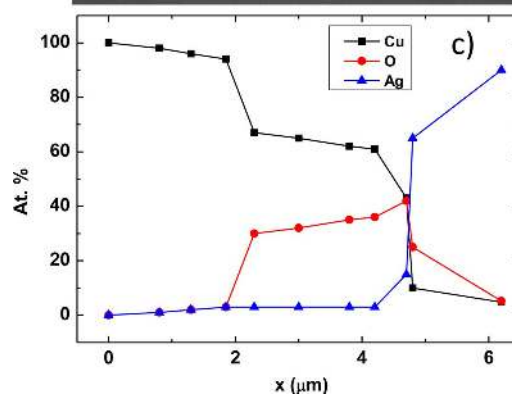
Fig. 4. Cross-sectional images of samples sintered at 200°C (a) and 350°C (b). An EDX element analysis is provided for sample sintered at 350°C (c).
