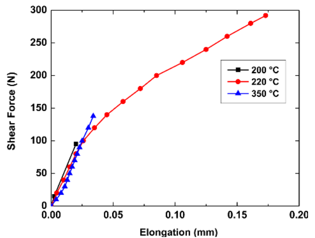
Fig. 5. Results of shear test for Cu/Ag/Cu joint samples sintered at different temperatures.
