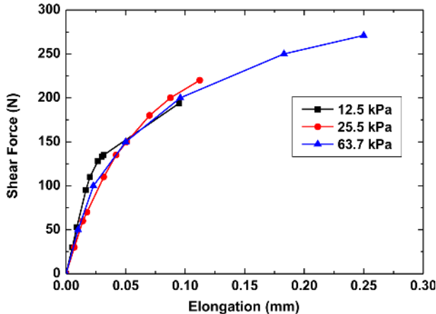
Fig. 6. Results of shear tests for Cu/Ag/Cu joint samples loaded by uniaxial pressure and sintered at 350°C in air.
