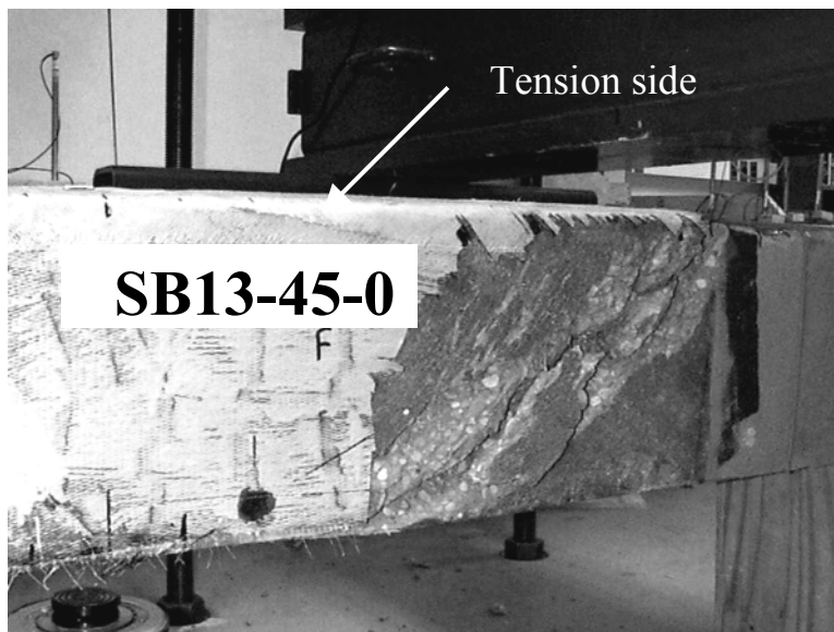
Figure 7: Failure Pattern of the Beam Bonded with CFRP Fabric Inclined at \pm 45^\circ ; Shear and Delamination of CFRP Fabric
