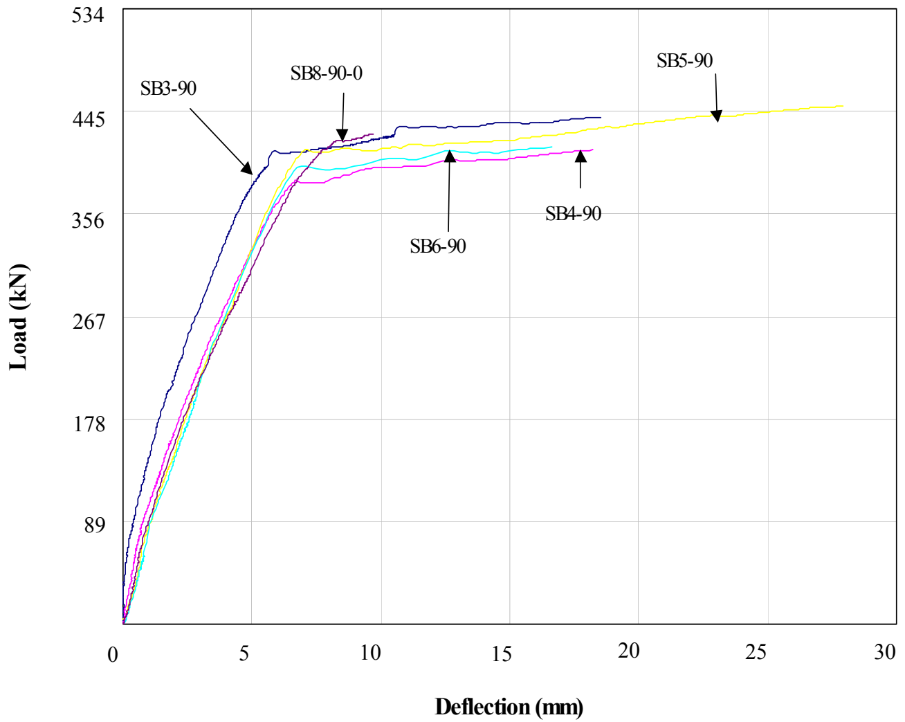
Figure 9: Load/Centerline Deflection Curves for Beams Wrapped with CFRP Fabric Inclined at 90°, and 90° with 0°
