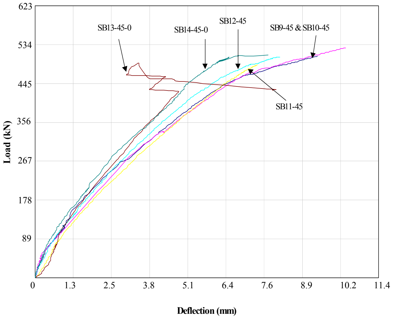
Figure 10: Load/Centerline Deflection Curves for Beams Wrapped with CFRP Fabric Inclined at 45°, and 45° with 0°
