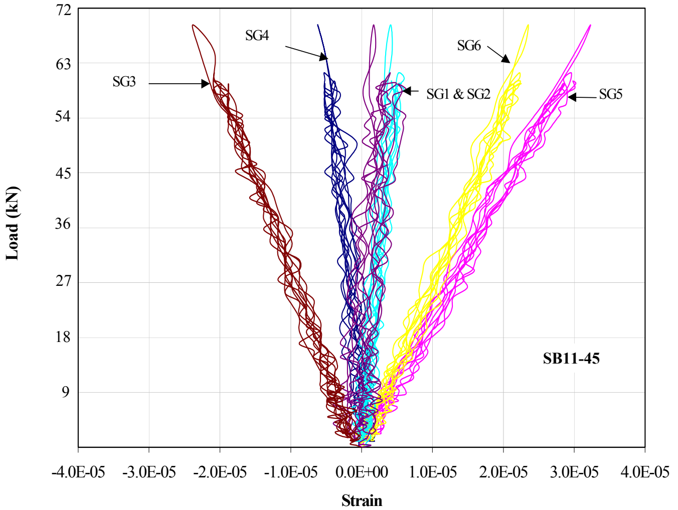
Figure 11: Typical Load/Strain Curves for Beams Wrapped with CFRP Fabric Inclined at \pm 45^\circ
