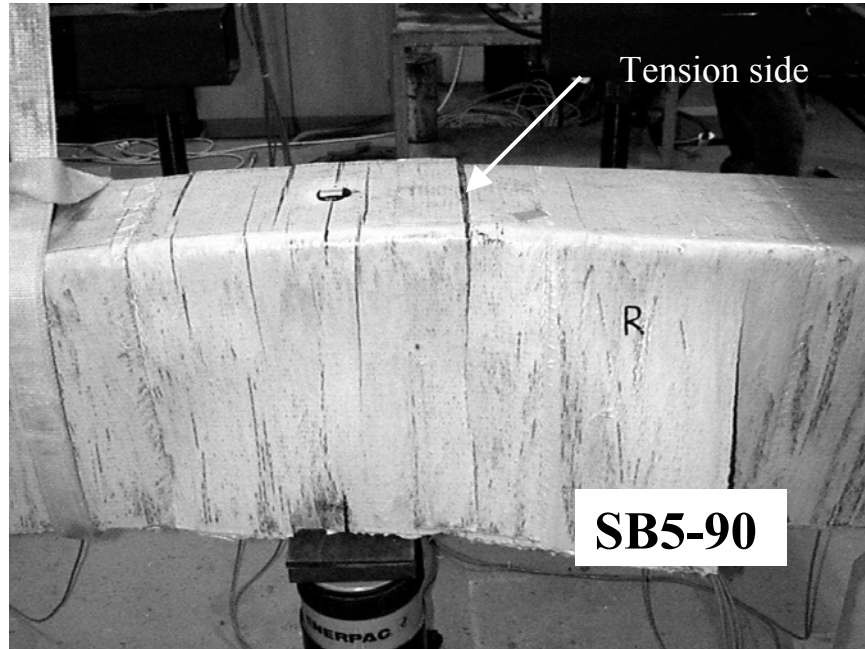
Figure 5: Failure Pattern of the Beam Bonded with CFRP Fabric inclined at 90°; Rupture and Delamination of CFRP Fabric
