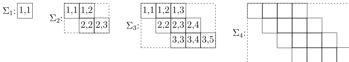
Figure 0.1: The diamond shapes \Sigma_m
