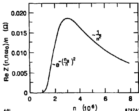
Figure 1. \text{Re } Z(n, n_{w0})/n versus n for the parallel-plate model, R = 149.5 m, h = 2 cm.
