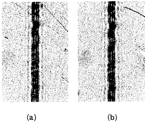
FIG. 2. (a) Fringe pattern due to biprism alone. (b) Pattern displaced by 2.5 fringe widths by field of type a' .
