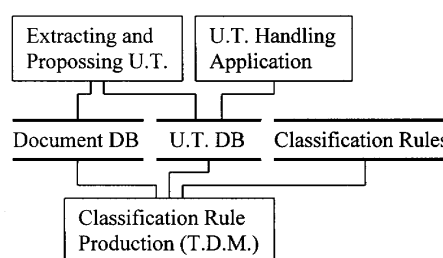
Figure 3: The architecture of Document Classification
