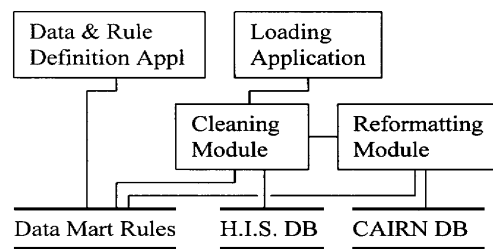
Figure 4: Data Mart Architecture.
