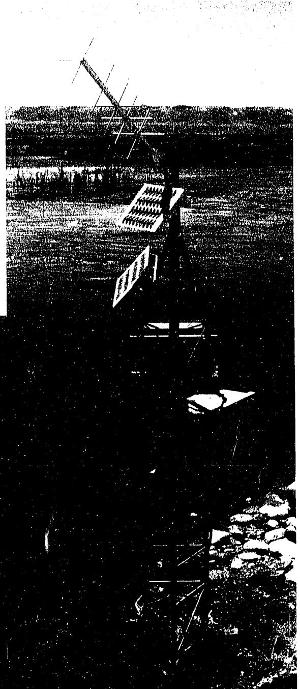
This remote water-level-monitoring station uses photovoltaics for charging storage batteries that supply electric power. Solar radiation data provide information for determining the size of the photovoltaic and battery system needed to supply remote stations like this with reliable electric service.
