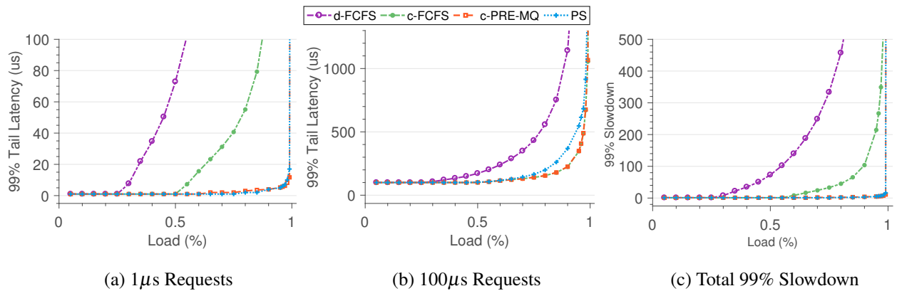
Figure 2: Simulation results for \text{Bimodal}(50 - 1, 50 - 100) for a 16-core system.
