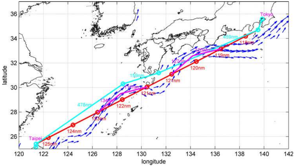
Figure 9. Ship routing laid over bin-averaged strong currents between Taipei and Tokyo. The red line represents the initial proposed straight route. The recommended magenta line takes advantage of strong, along-route currents, and cyan line avoids the Kuroshio on the return leg. See text for details.
