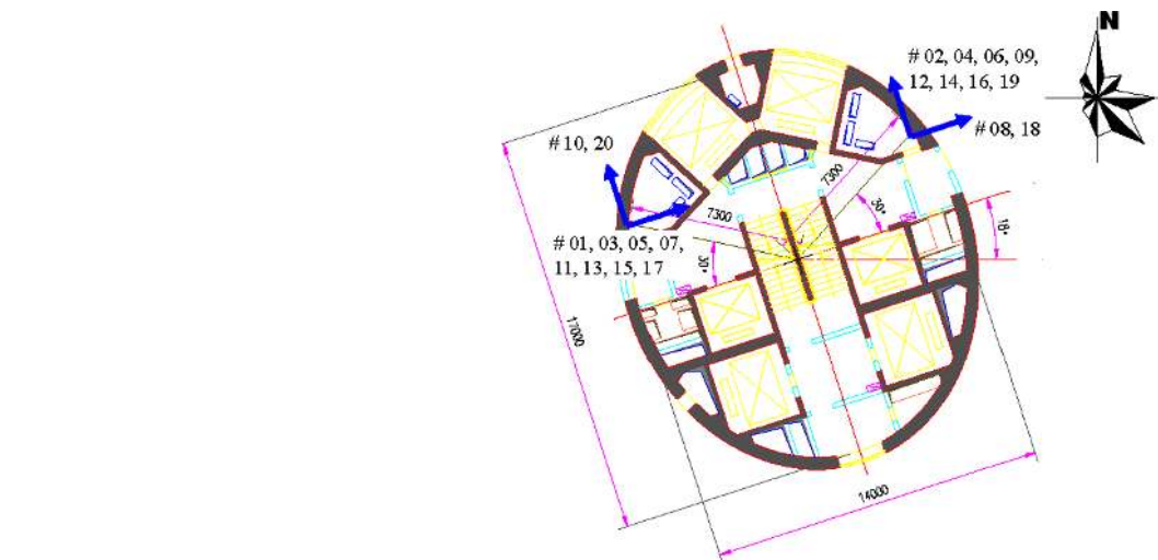
Fig. 6 Measurement positions and directions of accelerometers at different sections
