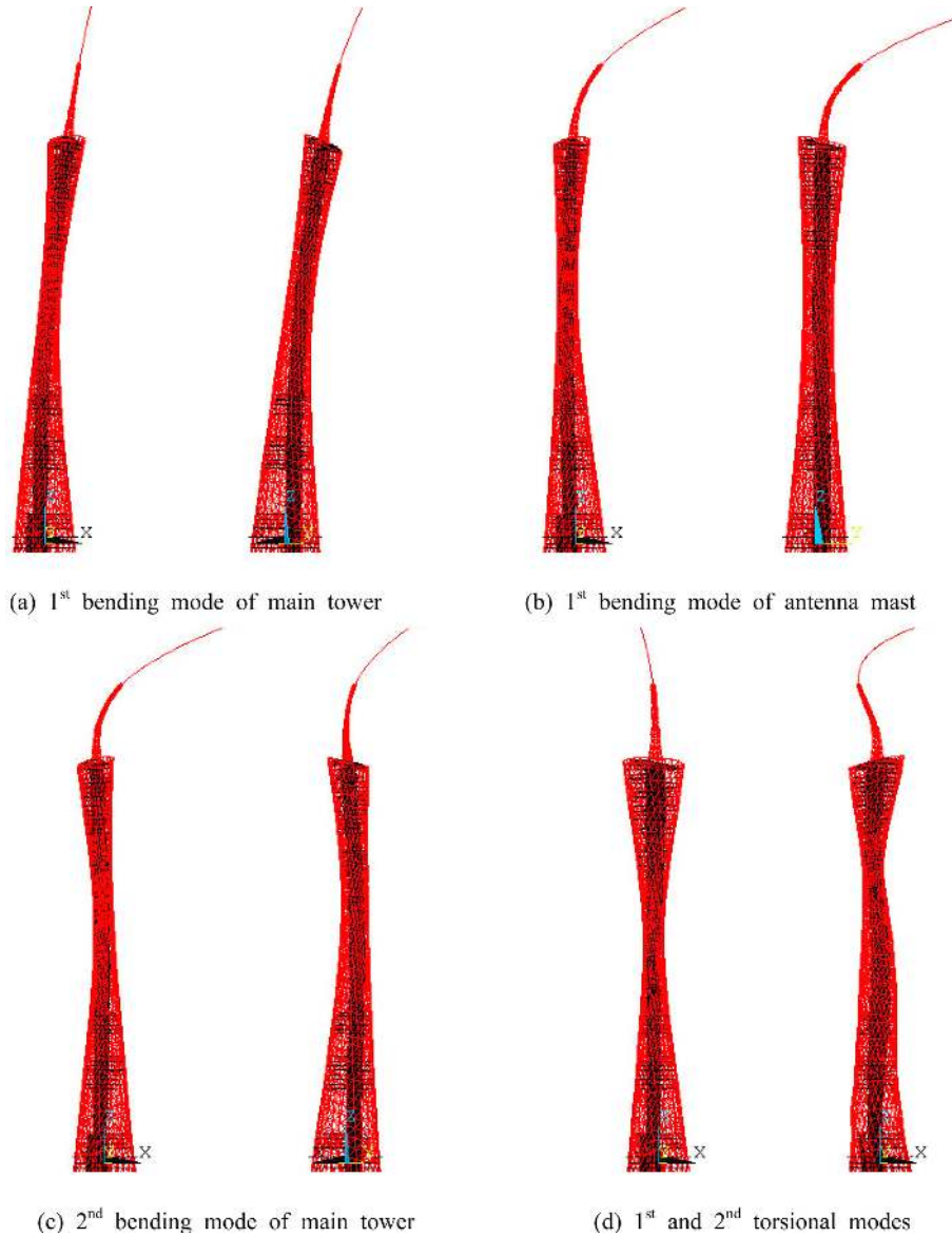
Fig. 2 Mode shapes obtained by full-scale FEM
