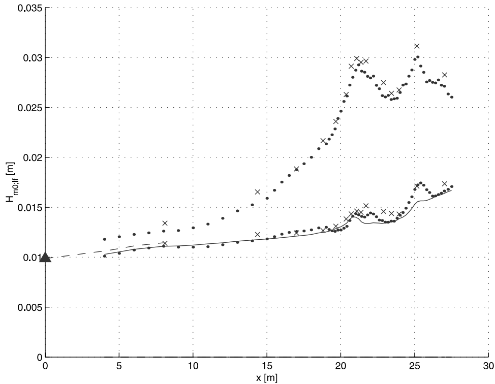
Figure 4. H_{m_0,lf} values for incoming (upper set of data) and outgoing (lower set of data) lf waves, based on array method (dots) and colocated method (crosses). Dashed curve: Green's law over approach slope, initiated with LHS62 solution in the constant depth portion (dark triangle). Drawn curve: Green's law initiated with outgoing wave height at x = 8 m.
