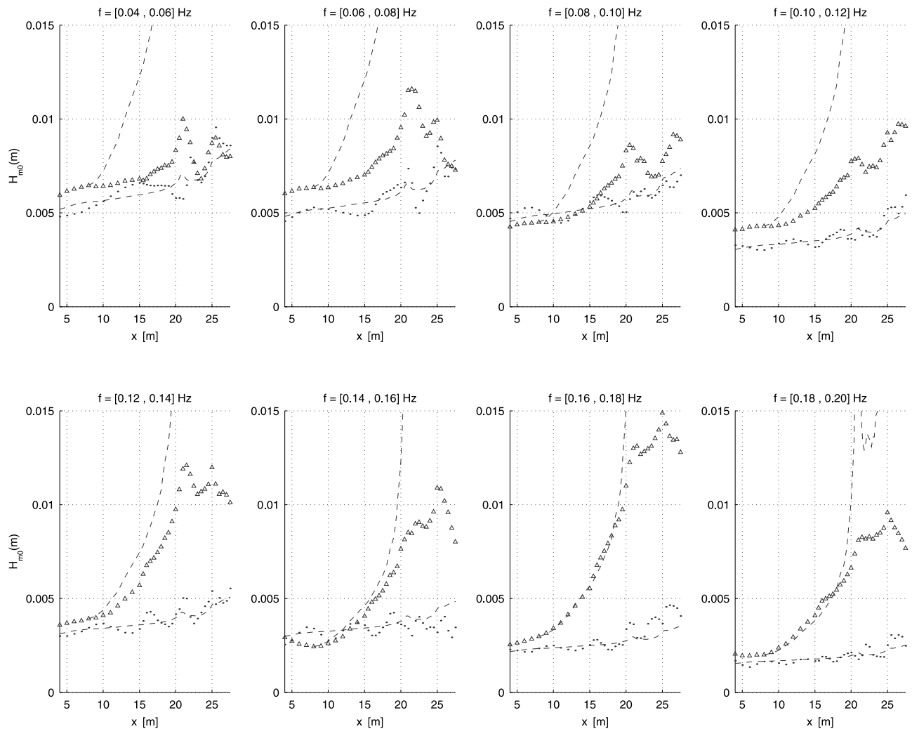
Figure 5. H_{m0} values of incoming (triangles) and outgoing (dots) lf waves for different frequency bands. Lower dashed curve: Green ( H \sim h^{-1/4} ), fitted to outgoing wave heights in the zone offshore from x = 20 m; upper dashed curve: LHS62 asymptote ( H \sim h^{-5/2} ), initiated with wave height at x = 8 m.
